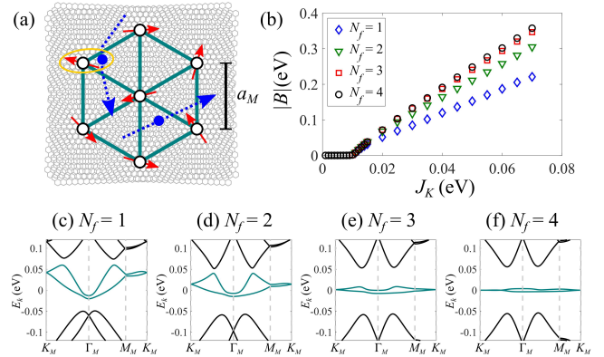
FIG. 1. Kondo lattice model for MATBG. (a) The real-space structure. Local moments (red arrows) are located at the AA stacking registries and form a triangular lattice with a lattice constant a_M . The delocalized c fermions (blue dots) interact with these local moments. (b) The Kondo hybridization amplitude as a function of J_K with different values of N_f . The results are obtained by solving Eqs. (6), (7), and (8) with a 30 \times 30 momentum mesh in each mBZ. (c)-(f) Quasiparticle dispersion of \eta = +1 for J_K = 0.03 eV with different N_f . (\nu_f, \nu_c) = (N_f - 4, 0) in these plots. The mini bands are highlighted with green color.
