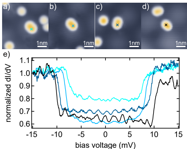
Figure 3. Antiferromagnetically coupled Mn dimers (oval structures) in different locations relative to the moiré structure. a-d) STM topographies of dimers (a) on the maximum, (b) close to the maximum, (c) further from the maximum, and (d) at the minimum of the moiré structure. e) dI/dV spectra acquired on the dimers shown in (a-d), with colors matched to the crosses in (a-d). Topographies recorded at 100 mV, 20 pA, setpoints of the recorded spectra 20 mV, 1 nA (b), 20 mV, 3 nA (a) and 15 mV, 3 nA (c), (d). Spectra are normalized for clarity.
