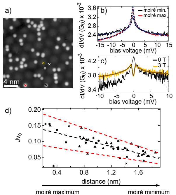
Figure 1. Variation of the Kondo coupling across the moiré structure. a) STM topography of Mn atoms on the moiré structure of \text{MoS}_2 on Au(111) (recorded at 100 mV, 20 pA). A moiré maximum (yellow), an hcp and fcc minimum (white) are indicated by crosses. b) dI/dV spectra taken on Mn atoms adsorbed close to a moiré maximum (red) and a moiré minimum (black), locations indicated in (a). Dashed lines show fits using a code based on Ref. [27]. The fits yield a (dimensionless) adatom-substrate exchange J\nu_0 of -0.080 (red) and -0.049 (black). c) dI/dV spectra on a Mn atom on a moiré minimum at 0 T (black) and 3 T (orange). The zero-bias resonance splits at 3 T (fit: dashed line). [Spectra recorded at a setpoint of 15 mV, 3 nA (panel b) and 10 mV, 3 nA (panel c)]. d) Values of J\nu_0 obtained from fitting dI/dV spectra (keeping T_0^2 = 0.000415 constant, as obtained from a best fit with B -field) on atoms at various positions within the moiré superstructure. Symbols indicate different measurement sets. The black dashed line is a linear guide to the eye through the data points. The red dashed lines are corresponding lines obtained from fits using different tunnel couplings T_0^2 . The upper line corresponds T_0^2 = 2.635 \times 10^{-4} and the lower line to T_0^2 = 5.6 \times 10^{-4} . These boundary values have been determined from error margins of fits at 3 T.
