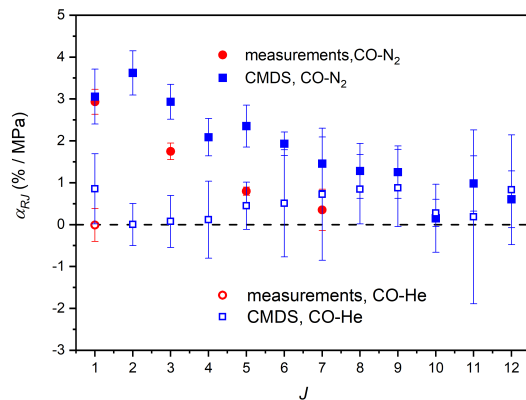
FIG. 2. Intensity-correction slopes obtained from measured (circles) and computed (squares) spectra versus the lower-state rotational quantum number J for RJ lines for CO-N 2 (full symbols) and CO-He (open symbols).
