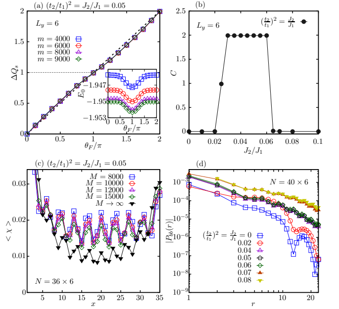
FIG. 2. Identifying the TSC phase and phase transitions along (t_2/t_1)^2 = J_2/J_1 . (a) Spin pumping simulation by adiabatically inserting flux \theta_F for J_2/J_1 = 0.05 . m is the U(1) bond dimension. By inserting a flux quantum, we obtain the Chern number C = \Delta Q_s \approx 2 with the error smaller than \pm 0.03 . The inset shows the flux dependence of ground-state energy per site E_0 . (b) Coupling dependence of the obtained Chern number with m = 8000 . (c) Spin chiral order \langle \chi \rangle = \langle \hat{\mathbf{S}}_i \cdot (\hat{\mathbf{S}}_j \times \hat{\mathbf{S}}_k) \rangle of the triangles in each column versus the column position x for J_2/J_1 = 0.05 . M is the SU(2) bond dimension. (d) Double-logarithmic plot of the pairing correlation |P_{bb}(r)| obtained with M = 12000 .
