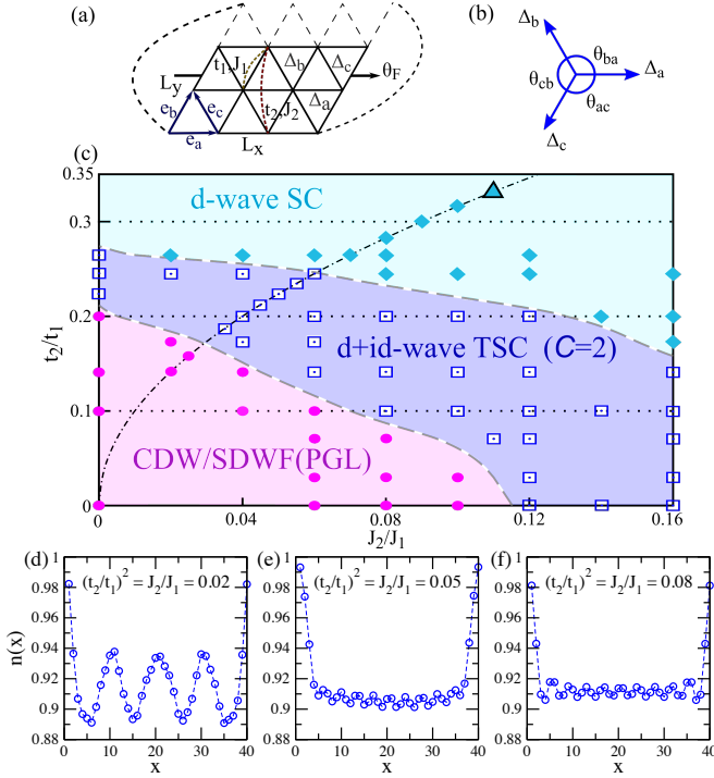
FIG. 1. Global quantum phase diagram. (a) Schematic figure of the triangular t - J model with the NN and NNN hoppings t_1, t_2 and spin interactions J_1, J_2 . \theta_F is the magnetic flux threading in the cylinder. \Delta_{a,b,c} define the pairing order parameters of the NN bonds along the e_{a,b,c} directions. (b) The relative phases between \Delta_\alpha = |\Delta_\alpha|e^{i\theta_\alpha} ( \alpha = a, b, c ), defined as \theta_{\alpha\beta} = \theta_\alpha - \theta_\beta . (c) The quantum phase diagram obtained on the L_y = 6 cylinder with doping level \delta = 1/12 . We identify a pseudogap-like (PGL) phase with CDW/SDWF, a d + id -wave TSC phase, and a d -wave SC phase. The dotted dashed line denotes J_2/J_1 = (t_2/t_1)^2 . The symbols mark the studied parameters, and the cyan triangle marks the studied parameter in Ref. [55]. (d-f) The charge density profile in the three phases. n(x) is the charge density per site in each column x , obtained on the 40 \times 6 cylinder with M = 12000 .
