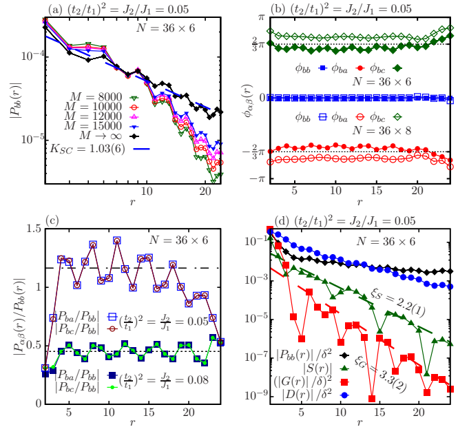
FIG. 5. Correlation functions for (t_2/t_1)^2 = J_2/J_1 = 0.05 in the TSC phase using the extrapolated data. (a) Double-logarithmic plot of the pairing correlations |P_{bb}(r)| obtained by keeping different SU(2) bond dimensions. The extrapolated correlations decay algebraically with K_{SC} = 1.03(6) . (b) d + id -wave pairing symmetry identified by the phase differences of pairing correlations on the L_y = 6 ( 8 ) cylinder using bond dimensions M = 15000 ( 20000 ). (c) The ratios of the magnitudes of the pairing correlations at different bonds. The dashed dotted line indicates the averaged ratio of 1.2(1) for TSC phase. The dotted line indicates the averaged ratio of 0.45(5) for the d -wave SC phase. We choose r \leq L_x/2 to calculate the averages to minimize the boundary effect. (d) Comparing the correlations which are rescaled with doping ratio. The fittings give \xi_S = 2.2(1) and \xi_G = 3.3(2) . We choose x_0 = L_x/4 and fit the data to the distance r = L_x/2 to avoid boundary effect.
