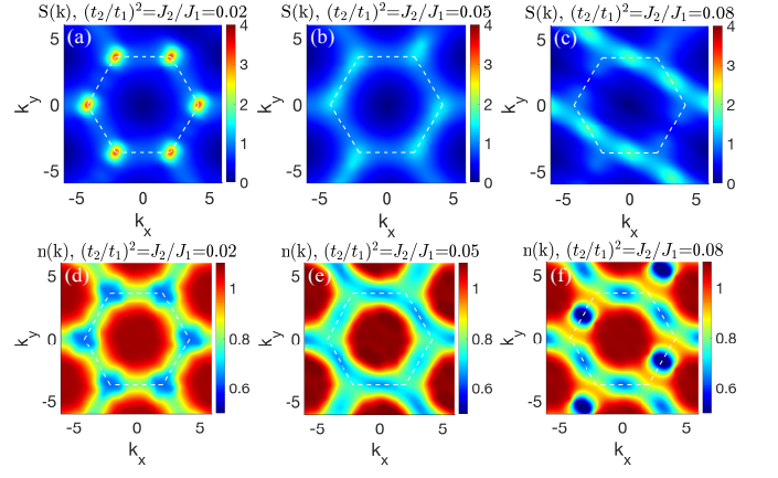
FIG. 3. Spin structure factor S(\mathbf{k}) and electron density in momentum space n(\mathbf{k}) in the three phases. The results are obtained using the middle N_m = 24 \times 6 sites of a long cylinder, which are calculated with M = 12000 and well converged. The dashed hexagon denotes the Brillouin zone.
