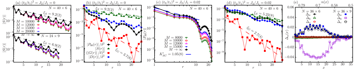
FIG. 4. Correlation functions and SC orders in the CDW/SDWF phase with extrapolated M \rightarrow \infty data for (a-d). (a) Logarithmic-linear plots of the spin correlations on the 40 \times 6 and 24 \times 9 cylinders, with the correlation length \xi_S = 9.2(2) ( 6.9(2) ) for L_y = 6 ( 9 ). The number in bracket gives the standard deviation from linear fitting. (b) Comparing correlations which are rescaled with doping ratio for a direct comparison. The fittings give \xi_S = 9.2(2) and \xi_G = 3.7(6) . (c) Double-logarithmic plot of pairing correlation |P_{bb}(r)| . The extrapolated results with r \leq 10 can be fitted algebraically with K'_{SC} = 1.05(8) . (d) Comparing correlations where the fittings give \xi_S = 5.22(8) and \xi_G = 2.7(4) . We choose the reference site at x_0 = L_x/4 for demonstrating correlations. (e) Different SC orders \Delta_\alpha versus each column x for a system in grand canonical ensemble with M = 8000 and the averaged electron density n(x) . The coupling parameters are the same as (d). A varying chemical potential \mu_i = \mu(x) = \mu_0 + x/L_x(a + b(x/L_x)) is used to adjust the range of n(x) .
