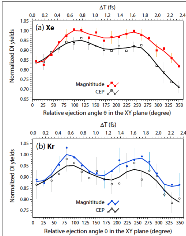
Figure 3 Resolving the direction of time in 2eAS with absolute CEP measurements in (a) xenon and (b) krypton. Comparison between time transients obtained with employing momentum magnitude or absolute CEP as the discriminators.
