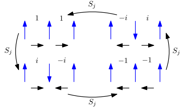
FIG. 3. The action of S_j on domain wall states in the SPT edge theory: S_j shifts the domain wall measured by C_{j-1}^\dagger C_j by i and the domain wall measured by C_j^\dagger C_{j+1} by -i . Here, j labels the spin in the middle of each 5-spin configuration.
