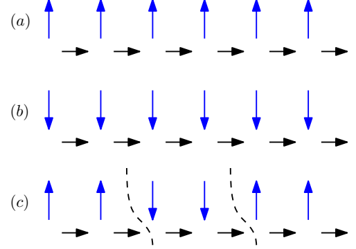
FIG. 1. (a)-(b) The two degenerate ground states of the Hamiltonian (2) that spontaneously breaks \mathbb{Z}_{2a} . The blue arrows represent the \sigma_j spins and the black arrows represent the \tau_{j+1/2} spins. Both states are eigenstates of U_b with eigenvalue +1 . (c) Domain walls occur at the boundaries between these states. A state with two \mathbb{Z}_{2a} domain walls (indicated by the dashed lines) has eigenvalue -1 under U_b , meaning two \mathbb{Z}_{2a} domain walls fuse to a \mathbb{Z}_{2b} charge.
