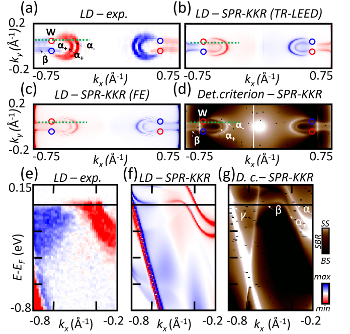
FIG. 2. LD, CD and determinant criterion in VUV regime on TaP. (a) shows experimentally measured LD using the same experimental geometry as described in Fig. 1(b). Calculated LD with TR-LEED final state (b) and FE final-state in (c). The determinant criterion plot for the corresponding CECs is provided by the one-step model (KKR) method in (d). (e) and (f) represent the corresponding E(k_x) cuts marked by the dashed green line in (a) and (b). (g) shows the E(k_x) plot of the corresponding determinant criterion. The spoon- and neck-shaped features are labeled \alpha_+ , \alpha_- , and \beta correspondingly. The circles denote projected WP. Red and blue colors of WPs indicate opposite chirality.
