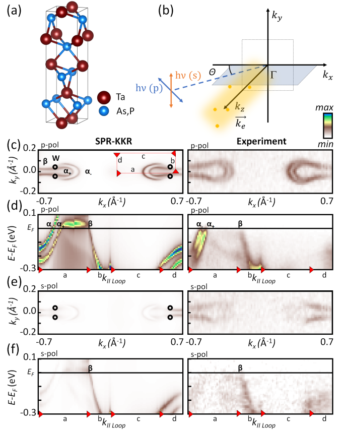
FIG. 1. (a) Crystal structure of TaP and TaAs. (b) Geometrical configuration used both in experiment and SPR-KKR calculations. p- or s-polarized VUV ( h\nu = 105eV ) photons are focused onto a freshly cleaved bulk crystal at an angle of incidence of \Theta = 17^\circ ( 33.25^\circ for the VUV data in Fig. 3). The figures (c) and (e) show constant energy contours (CECs) at E_F taken with p- and s-polarized VUV light respectively. For both CECs in (c) and (e), a corresponding band structure cuts (d) and (f) were extracted in the anticlockwise direction starting along the k_x direction as represented by a-b-c-d sequence in (c). One-step model photoemission intensity calculations on TaP are on the left and experimental data are on the right.
