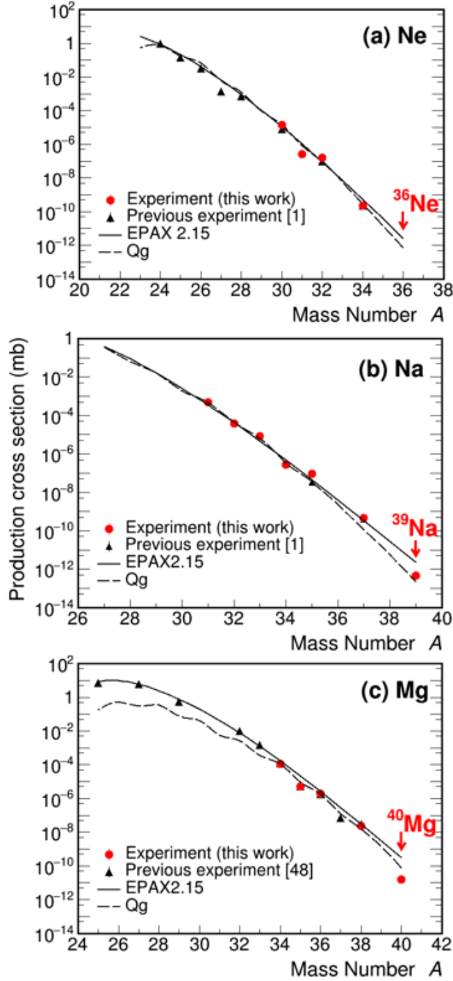
FIG. 2. Measured production cross sections are shown as a function of mass
