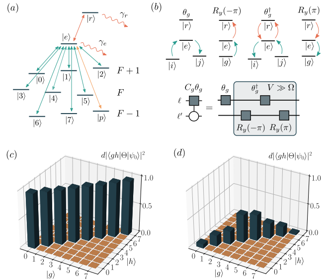
FIG. 2. Qudit encoding and native gates: (a) Atomic level structure serving as a Q_8 -register, where the d = 8 group basis elements are encoded into different hyperfine manifolds. Single and two-qudit gates are performed holonomically using the auxiliary ground-state level |p\rangle and excited states |e\rangle and |r\rangle , with corresponding decay rates \gamma_e/\gamma_r . (b) Controlled-permutation gate C_{\theta(g)}^{\ell\ell' \to \ell}(g) as a sequence of four single qudit-gates in the blockade regime. Quantified by the maximally-entangled state obtained after applying \Theta_{\ell|\ell'} to |\Psi_0\rangle , implemented through the (c) qudit and (d) qubit protocols [see the circuit in Fig. 1(c)] using the same experimental parameters (see main text), we obtain a state fidelity of 99.6% and 21.4%, respectively, demonstrating the clear advantage of a qudit-based decomposition.
