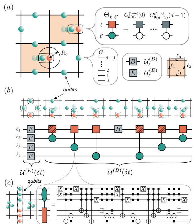
FIG. 1. Gauge field dynamics on qudit vs. qubit quantum simulator: (a) Our proposal employs Rydberg atoms trapped in optical tweezers, arranged on the links \ell of a hypercubic lattice. Each atom encodes a qudit using d internal levels, where single-qudit gates are realized holonomically. To implement the entangling two-qudit gate \Theta_{\ell|\ell'} we first bring pairs of atoms within the Rydberg blockade radius R_b . (b) First order decomposition of a Trotter step, including the four-qudit plaquette interaction, into the native atomic gates U_{\ell}^{(E/B)} and \Theta_{\ell|\ell'} . (c) For comparison, we show a qubit-based circuit decomposition of \Theta_{\ell|\ell'} for the Q_8 group, where the number of required atoms is increased by a factor \log_2 8 = 3 , leading to much lower gate fidelities, while our qudit-approach enables a faithful simulation [see Figs. 2(c) and (d)].
