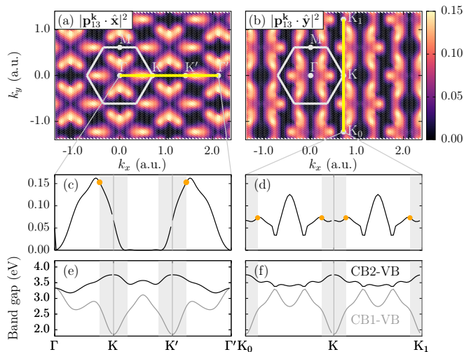
FIG. 4. Modulus squares of the recombination dipoles along (a) \hat{x} ( \alpha = 30^\circ ) and (b) \hat{y} ( \alpha = 0^\circ ) directions in a.u. The gray hexagon traces the 1st Brillouin zone. Panels (c) and (d) plot the same as (a) and (b), but along paths in reciprocal space marked by the yellow lines. Panel (e) and (f) show the band gaps along these paths, with the gray (black) curve between CB1 (CB2) and the VB. The areas marked by gray indicate regions accessible by electron-hole pairs created at the K point, with maximum excursions \pm A_0 , and the orange dots in (c) and (d) highlight the maximum values in these regions.
