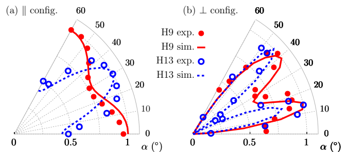
FIG. 2. Experimental and simulation \alpha -dependent HHG yields with a 3.7 \mu\text{m} driver, for the (a) parallel and (b) perpendicular configurations. The yields are normalized to the maximum.
