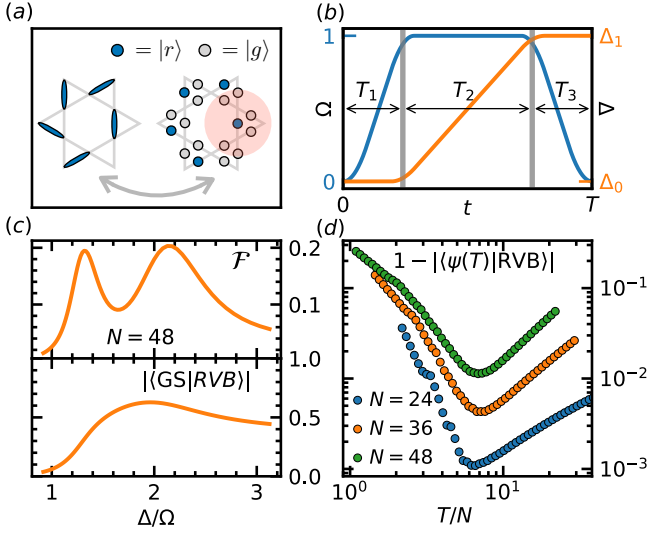
Figure 1. (a) Mapping between a dimer model on the kagome lattice and the Rydberg atoms system on the ruby lattice. When R_b \gtrsim 2a (shaded red circle) the Rydberg constraint is equivalent to the dimer constraint. (b) Schematic representation of the adiabatic state preparation protocol. The vertical grey lines separate the three stages of the preparation process: ramp-up of \Omega and \Delta , and ramp-down of \Omega . (c) Top: Groundstate fidelity susceptibility \mathcal{F} = (1 - |\langle \text{GS}(\lambda) | \text{GS}(\lambda + d\lambda) \rangle|) / d\lambda with \lambda = \Omega/\Delta and d\lambda = 0.0025 . Bottom: RVB overlap with the groundstate of the Hamiltonian Eq. (1). (d) Overlap between the dynamically prepared state and the RVB state as a function of the total sweep time T rescaled with the number of atoms N , for \Delta_0 = -5 , \Delta_1 = 1.5 , T_1 = T_3 = 0.1T and T_2 = 0.8T .
