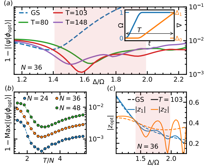
Figure 2. (a) Overlap between the dynamically prepared state during the sweep (depicted in the inset) and the ansatz Eq. (2), optimized over the variational parameters z_1, z_2 for various sweep times T , for a periodic cluster of N = 36 atoms. The dashed line is the optimized overlap with the instantaneous groundstate ( T = \infty ). The shaded red region delimits the topological phase in the groundstate. (b) Maximal overlap obtained during the sweep when 1 \lesssim \Delta/\Omega \lesssim 2 , for different N , as a function of the total sweep time rescaled by N [27]. (c) Optimal absolute values for the variational parameters z_1, z_2 in the ansatz state during a semi-adiabatic sweep with T = 103 (solid line) and on the ground state (dashed line) for N = 36 .
