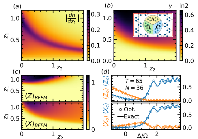
Figure 3. (a) Derivative of the density w.r.t. the parameter z_1 , computed from the TN representation of the ansatz Eq. (2) on an infinite cylinder of circumference L=6 tensors. (b) Topological entanglement entropy \gamma of the ansatz computed on the finite cluster of N=48 sites depicted in the inset. (c) Diagonal and off-diagonal BFFM order parameters on the infinite cylinder of circumference L=6 . (d) Expectation values of open and closed string operators obtained during the dynamical preparation (solid lines) and from the optimized ansatz (empty markers) for N=36 and T=65 .
