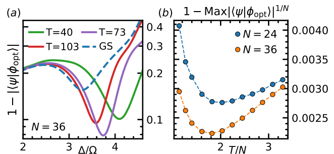
Figure 4. (a) Optimized overlap between the ansatz Eq. (2) (without projector \mathcal{P} ) and the state prepared through the sweep depicted in the inset of Fig. 2(a) for different total sweep times T . The dynamics is generated by the full Rydberg Hamiltonian Eq. (1) with R_b = 2.4a . (b) Maximal fidelity per site obtained during the sweep as a function of the total sweep time T rescaled by the number of atoms N .
