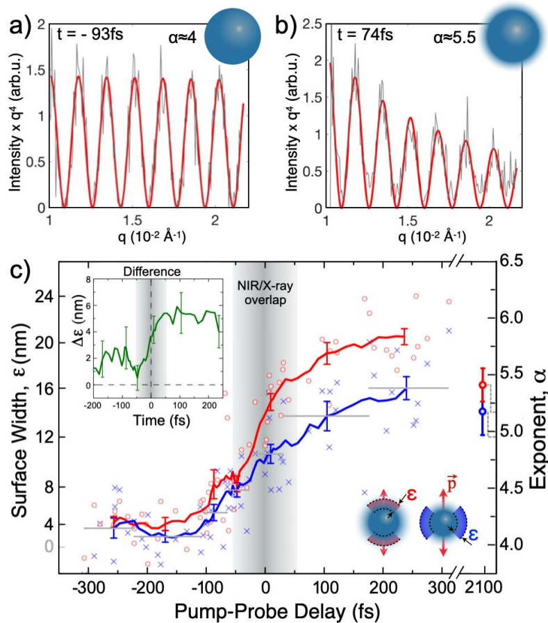
Figure 2: a), b) Power-law fits (red) of azimuthally integrated scattering patterns (gray), indicating exponents of a) \alpha \approx 4 before and b) \alpha \approx 5.5 after the laser-droplet interaction. Intensities are scaled by q^4 for improved clarity. c) Temporal evolution of the exponents \alpha (right) and corresponding surface widths \epsilon (left) for 90^\circ wide angular ranges parallel (red) and perpendicular (blue) to the NIR polarization axis. Circles and crosses mark individual data points, lines represent 10-point moving averages. Note that the exponent values on the right ordinate apply to all data points except those at 2.1 ps delay, whose values are indicated by the dotted gray lines. The left ordinate applies to all data. Exemplary vertical error bars indicate uncertainties of the mean values, horizontal gray lines indicate corresponding 10-point averaging ranges. The inset shows the average difference between parallel and perpendicular surface widths (green). Gray-shaded areas indicate the nominal NIR/X-ray pulse overlap.
