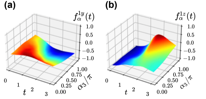
FIG. 2. Control of the family of arbitrary single-qubit rotations U_\alpha^1 defined in Eq. (3) with the Hamiltonian in Eq. (1). The framework is successfully trained to implement any of the target rotations, resulting in an average infidelity of \bar{\mathcal{I}} = 2 \times 10^{-4} (assessed on new targets not seen during training). To visualize the controls produced by the NN, \alpha_1 and \alpha_2 are kept fixed to a value of 3\pi/4 and \alpha_3 is varied in the range [0, \pi] . The amplitudes of the two control fields f_\alpha^{1y} (panel a), and f_\alpha^{1z} (panel b) produced by the NN are plotted as a function of both the time t and \alpha_3/\pi .
