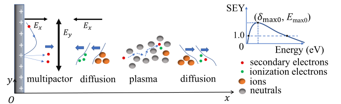
FIG. 1: Schematic of the system for multipactor induced ionization breakdown in fully kinetic particle-in-cell simulations. The small zoomed plot qualitatively shows the secondary electron yield (SEY), \delta , as a function of electron impact energy for normal incidence.
