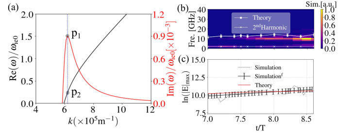
FIG. 4: (a) Theoretical dispersion relationship solution, real and imaginary part of \omega , \text{Re}(\omega) (black line) and \text{Im}(\omega) (red line), versus k , and the blue dashed line indicates the maximum \text{Im}(\omega) . (b) The time varying frequency spectrum (color bar from simulation) of the normal electric field E_x over time range of 7.0–8.6 rf periods. The color bar gives the relative strength of the magnitude of the Fourier transform of the normal electric field. The time window is 64% of the rf period, with a 78% overlap between successive windows. The white rectangle line shows the theoretical calculation oscillation frequency. (c) The amplitude of the fast oscillation as a function of time in simulation (black dashed line), its linear fitting (black line) and theory (red line).
