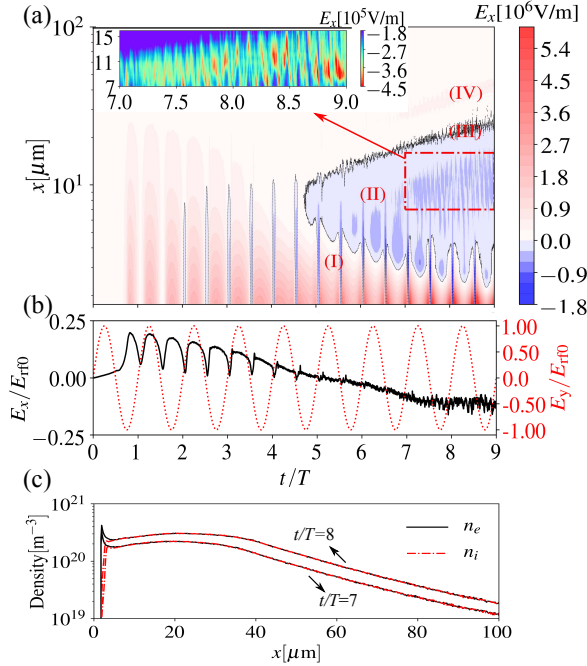
FIG. 2: Spatiotemporal plots of the (a) normal electric field, E_x , (b) the normalized rf electric field (red dashed line), E_y/E_{rf0} , and normal electric field, E_x/E_{rf0} at x = 12\mu\text{m} , (c) the spatial plots of electron and ion density at t/T = 7, 8 .
