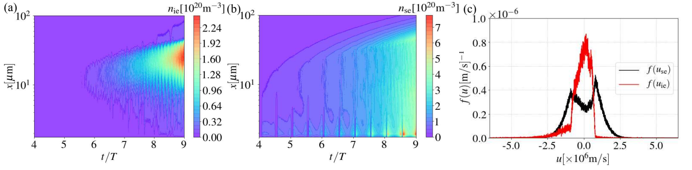
FIG. 3: The spatiotemporal plots of the (a) electron density from ionization impact and (b) secondary electron density from the surface emission; (c) the velocity distribution functions at x = 12\mu\text{m} of the ionization and secondary electrons normalized to each species density.
