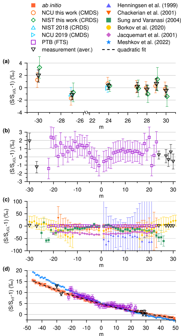
FIG. 1: Summary of present experimental and theoretical results for the (3–0) band of ^{12}\text{C}^{16}\text{O} , and comparison to literature data. Panel (a): Comparison of NCU and NIST intensity measurements, S , for high- J lines, expressed as (S/S_{UCL} - 1) , where S_{UCL} are the present theoretical intensities. The black triangles represent weighted averages of the measurements. NCU 2019 indicates the measurement from Ref. [3] and NIST 2018 indicates a prior measurement conducted at NIST in 2018. Note the break in the x axis. Panel (b): Analogous comparison of low- J PTB intensity values and average high- J values from panel (a). Panel (c): m dependence of (S/S_{UCL} - 1) where S corresponds to literature data [35–39] (closed symbols) and present measurements (open symbols). Note the extended range of the y -axis scale compared to the other panels. Panel (d): m dependence of (S/S_{HT} - 1) where S corresponds to experimental (open symbols) and theoretical (orange squares) intensities from this work as well as semi-empirical intensities from Ref. [40] (blue stars). S_{HT} are values from HITRAN 2020 [41] intensities scaled to 100 % ^{12}\text{C}^{16}\text{O} . The dashed line is a second-order polynomial fit of the ratio (S_{UCL}/S_{HT} - 1) versus m . This function, f(m) = a_0 + a_1m + a_2m^2 provides a convenient mapping of the HITRAN 2020 intensities on to the present theoretical values. Here, a_0 = 4.865 %, a_1 = -0.1789 %, and a_2 = 0.001020 %. Note the differing x axes for the various panels.
