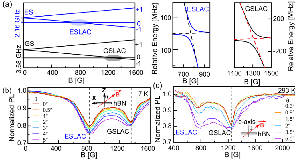
FIG. 4 (a) Energy level diagram of V_B^- centers under a tilted external magnetic field (2 degrees) with respect to the c -axis of the sample. Two LAC magnetic fields between m_s = 0 and m_s = -1 are highlighted in the blue shaded ellipse for the ES and the black shaded ellipse for the GS. The hyperfine interactions are not included in the simulation. Inserts show the zoomed crossing points near ESLAC (middle) and GSLAC (right). The relative frequencies are obtained by deducting the frequencies at 769 G and at 1307 G. In the simulation, D_{GS} = 3684 MHz, E_{GS} = 50 MHz, and D_{ES} = 2160 MHz, E_{ES} = 78 MHz are employed. Normalized magnetic field-dependent emission count rate at 7 K (b) and 293 K (c). The emission count rate is normalized to emission at 0 G for (b) and at 2200 G for (c). In (b), the angle is defined between the magnetic field in the X-Z plane and Z-axis. There is a B_y component due to the 2 degree sample tilting in the Y-Z plane. In (c), the alignment uncertainty is 0.05 degree.
