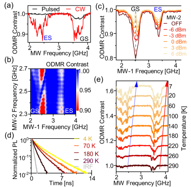
FIG.2 (a) ODMR spectra of V_B^- centers under pulsed laser/MW excitation (black) and CW laser/MW excitation (red). (b) GS-ODMR and ES-ODMR spectra (under an external B-field of 400 G) while sweeping an additional MW-2. The discontinuous signals of GS- and ES-ODMR are due to the large step size of MW2. (c) ES-ODMR at different MW-2 power. The MW-2 frequency is fixed at 2520 MHz. (d) Lifetimes of V_B^- centers at different temperatures. The IRF refers to the instrument response function that is much shorter than the lifetime. (e) Temperature-dependent GS- and ES-ODMR of V_B^- centers. The two arrows guide the shifting splitting energy as varying the temperatures.
