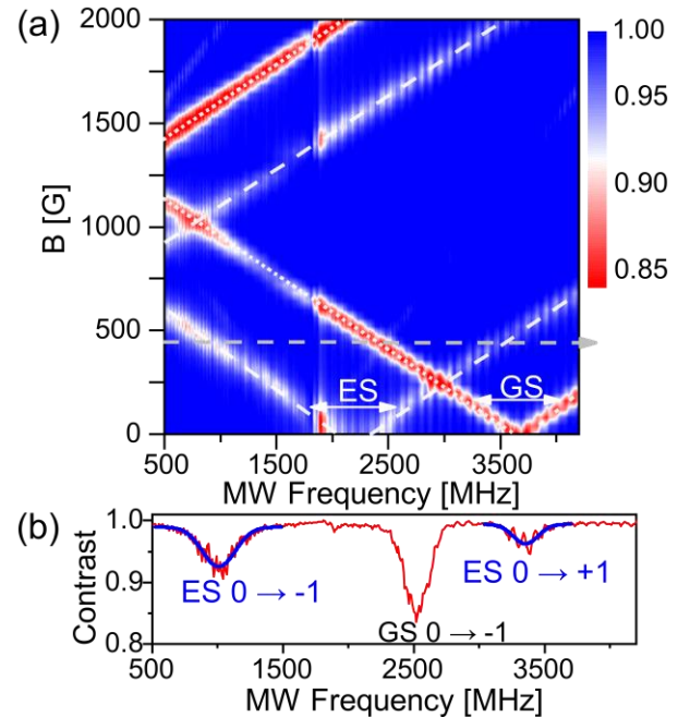
FIG.3 (a) Low-temperature B field-dependent GS- and ES-ODMR spectra. Dashed lines are the guidelines for ES-ODMR resonance frequency. The dotted line is the guide for GS. (b) Linecut ODMR spectra at 400 G, grey lines in (a). The blue curves are the Gaussian fit of the two ES transitions ( m_s = 0 to m_s = \pm 1 ).
