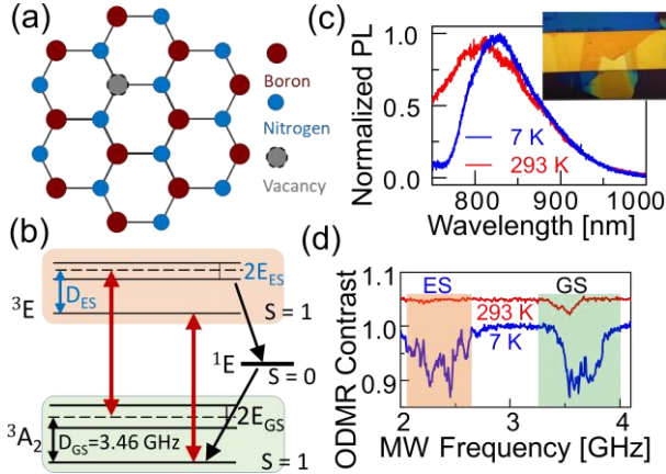
FIG. 1 (a) Schematic of a V_B^- defect in hBN. (b) Energy structures of V_B^- centers. It consists of a triplet ground state ( ^3A_2 ), a triplet excited state ( ^3E ), and a singlet state ( ^1E ). (c) Photoluminescence (PL) spectra of V_B^- centers excited with 532 nm light at 293 K (red) and 7 K (blue). Inset: the microscopic image of the exfoliated hBN on a 50 \mu\text{m} wide gold stripline. (d) GS-ODMR (light green shadow) and ES-ODMR (light gold shadow) of the V_B^- defects at 293 K and 7 K. The curves are vertically shifted for clarity.
