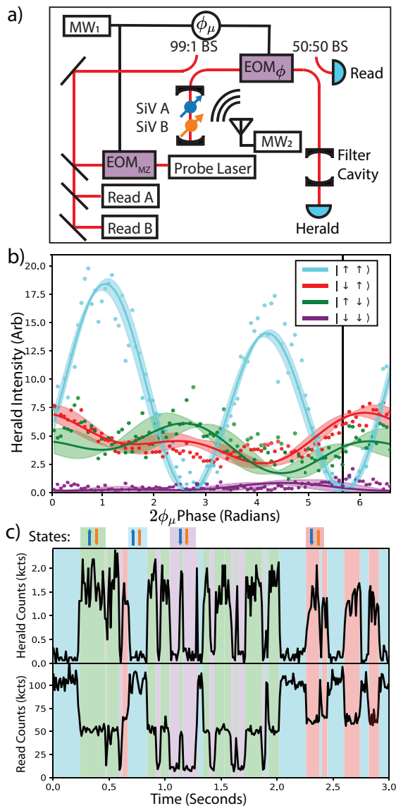
FIG. 2. (Color online) (a) Detailed experimental implementation. The relative phase \phi_\mu between the microwave drive ( MW_1 ) to the two modulators EOM_{MZ} and EOM_\phi sets the phase difference between the interferometer arms \Delta\phi = 2\phi_\mu . Readout is done sequentially with lasers at f_A and f_B by detecting a fraction of the light before the filter cavity. (b) Transmission to the heralding port vs interferometer phase for all SiV states |\downarrow\uparrow\rangle (red circles), |\uparrow\downarrow\rangle (green), |\uparrow\uparrow\rangle (cyan) and |\downarrow\downarrow\rangle (purple). Transmission predicted by a fit of the spin dependent reflection spectrum (Fig 1f) as solid lines with variance due to spectral diffusion given by shaded area. Phase and scaling are obtained by fitting the |\uparrow\uparrow\rangle state. The black vertical line indicates the phase used to collect the entanglement data. (c) Quantum jumps: Transmission through the filter cavity (top panel) and readout port (bottom panel) vs time with the entanglement heralding laser applied continuously. The filter transmission is a spin parity measurement, with high transmission corresponding to odd parity ( |\uparrow\downarrow\rangle or |\downarrow\uparrow\rangle ) highlighted with green or red background. Practically, we can distinguish these states by their slightly different transmission amplitudes through the readout port. Low transmission indicates either |\uparrow\uparrow\rangle (blue background) or |\downarrow\downarrow\rangle (purple background).
