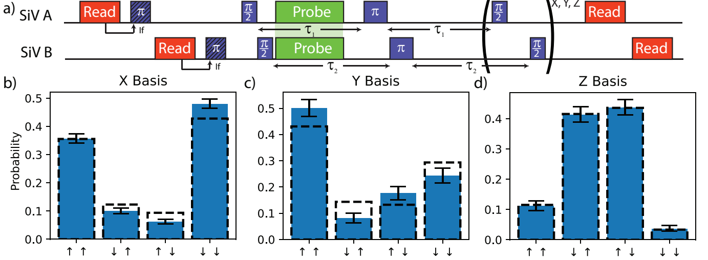
FIG. 3. (Color online) (a) The schematic of the sequence used to entangle the spins. Initialization and readout both apply 10 \mu\text{s} laser pulses at f_A or f_B . Counts are subsequently compared to a threshold to determine the state. Initialization follows this with a conditional \pi pulse. (b,c,d) Correlation statistics of the entangled state in XX, YY and ZZ spin bases. In the experimental data (blue), the measurement was taken with a heralding window of 200 ns. Dashed black lines are correlations predicted by a theoretical model. Error bars represent 68% confidence interval. Correlation data is composed of 407 Z basis heralds, 913 X basis heralds, and 222 Y basis heralds. [38]
