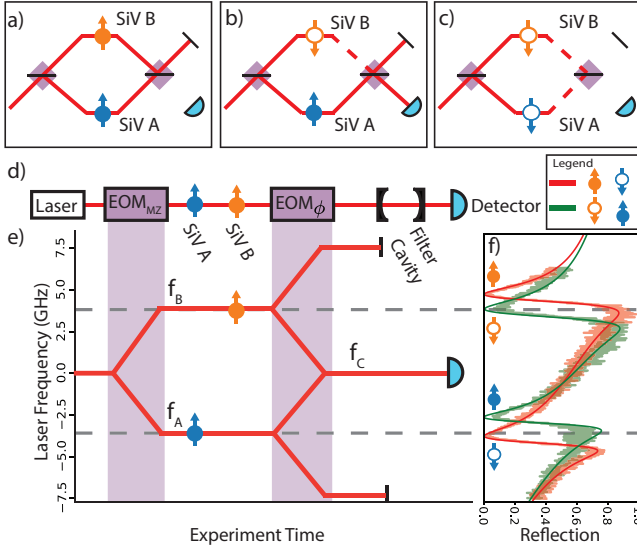
FIG. 1. (Color online) Optical entanglement of distinguishable emitters (a) An interferometer is tuned so that when no spin scatters light (full circle) photons leave only through the top port of the interferometer. (b) If just one spin scatters (empty circle) while the other reflects, light is split between the two output ports and the heralding detector receives photons. (c) If both spins scatter, no light leaves the interferometer. (d) The physical implementation of the protocol. The two SiVs act as spin-dependent mirrors. The relative phase between the microwave drive to the two modulators \text{EOM}_{MZ} and \text{EOM}_\phi sets the phase difference between the interferometer arms. (e) The Elitzur-Vaidman Gedanken-experiment implemented as a frequency domain interferometer. The y-axis shows the relative frequency of the relevant photonic modes in the protocol. Two EOMs (purple) play the role of beamsplitters. Detection of photons at the central frequency projects the SiVs into an odd parity state. (f) The spectrum of the two SiVs under investigation, when initialized in |\uparrow\uparrow\rangle (green) or |\downarrow\downarrow\rangle (red).
