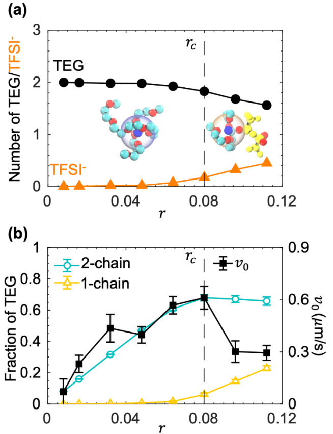
FIG. 3. (a) Average number of tetraglyme molecules (TEG, circles) and anions (TFSI ^- , triangles) in the coordination shell of each \text{Li}^+ cation, obtained from MD. A tetraglyme molecule or TFSI ^- anion is determined to coordinate \text{Li}^+ if one of its oxygen atoms lies within 0.3 nm of \text{Li}^+ . The insets, representative snapshots from simulations, depict the two-chain motif that dominates at low salt concentrations (left) and the one-chain motif that appears for r > r_c (right); Li is shown in dark blue, C is shown in cyan and O in red; within TFSI ^- , all atoms are shown in yellow except O in red. (b) Fraction of tetraglyme within the two-chain (open circles) and one-chain (open triangles) motifs, determined from MD. Solvent velocity measured by eNMR (filled squares) is overlaid using the right vertical axis, highlighting similar trends.
