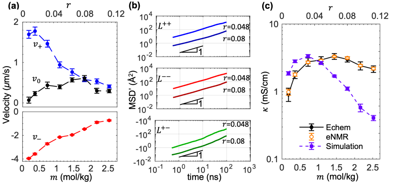
FIG. 1. (a) Average species velocities in LiTFSI/tetraglyme electrolytes ( r = [\text{Li}^+] / [\text{O}] ) measured by ^7\text{Li} , ^1\text{H} , and ^{19}\text{F} electrophoretic NMR (eNMR) at 30^\circ\text{C} : cation (blue), solvent (black) and anion (red). To highlight the smaller values of v_0 and v_+ , a separate vertical axis is plotted for these velocities compared to that for v_- . (See Fig. S4 for data plotted on same axis.) Velocities are in the lab frame of reference. All velocities reflect an applied electric field of 1 V/mm; measurements were performed at a range of electric fields and velocities were scaled to 1 V/mm. (b) Representative \text{MSD}' as defined in Eq. (6) calculated from MD simulations, for r = 0.048 (upper traces) and r = 0.08 (lower traces), corresponding to Onsager transport coefficients L^{++} (top), L^{--} (middle) and L^{+-} (bottom), which are extracted from the diffusive regime, i.e., the indicated timescale over which the slope equals one in the log-log scale. (c) Ionic conductivity from independent electrochemical and eNMR experiments (filled diamonds and open circles, respectively, which are nearly coincident), and predicted from MD simulations (filled squares).
