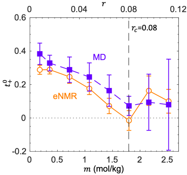
FIG. 2. Transference numbers in the solvent reference frame ( t_+^0 ) determined from eNMR (open symbols) and MD (filled symbols), using Eq. (2) and (5), respectively. The critical salt concentration, r_c = 0.08 , is indicated with a dashed line.
