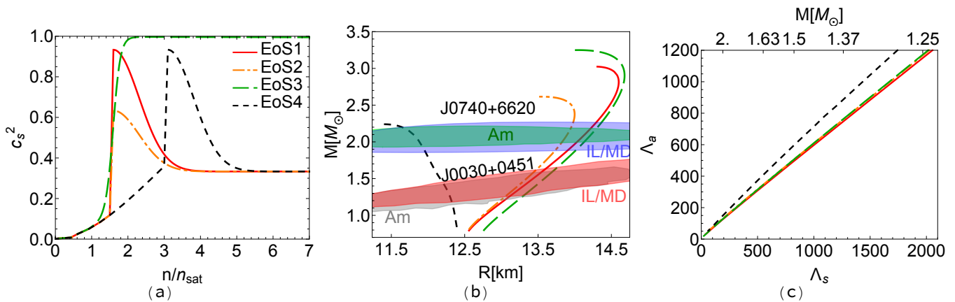
FIG. 1. (Color online) c_s^2 as a function of n/n_{\text{sat}} (panel a), mass-radius curves (panel b) and BLRs for a mass ratio of q = 0.75 (panel c) for 4 EoS models. Structure in the EoSs near saturation bends the mass-radius curves to larger radii, while still being consistent with the two NICER observations at 90% confidence (Amsterdam or Illinois/Maryland).
