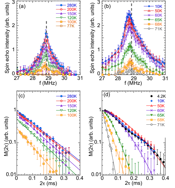
FIG. 2. Top: representative ^{79}\text{Br} NQR lineshapes observed (a) above and (b) below 75 K measured with a fixed \tau = 30 \mu\text{s} , corrected for the Boltzmann factor. The dashed vertical line marks the peak frequency ^{79}\nu_Q^{\text{Main}} = 28.85 MHz at 280 K. Bottom: spin echo decay curves M(2\tau) observed (c) above and (d) below 75 K. The fit in (c) is with M(2\tau) = M_0 \exp\{-(2\tau/T_2)^\beta\} with a fixed \beta = 1 , while \beta (\sim 1.3) was allowed to vary above 50 K in (d). The solid curves through the data below 50 K represent the best two component fit with an oscillatory term, M(2\tau) = M_0 [F \cos\{\omega(2\tau)\} \exp(-2\tau/D) + (1-F) \exp(-2\tau/T_2)^\beta] . The overall intensity of M(2\tau) in both (c) and (d) is corrected for the Boltzmann factor, and normalized to the M(2\tau = 0) value observed at 280 K.
