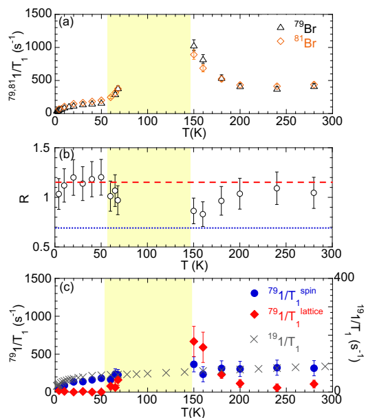
FIG. 4. (a) {}^{79,81}1/T_1 measured at the main peak. The results below 60 K were adopted from [15]. (b) The isotope ratio R = ({}^{81}1/T_1)/({}^{79}1/T_1) . Dashed and dotted horizontal lines mark R = 1.161 (dominated by spin fluctuations) and R = 0.698 (dominated by lattice fluctuations). (c) {}^{79}1/T_1^{spin} and {}^{79}1/T_1^{lattice} estimated from the results in (a). Also plotted using the right axis is {}^{19}\text{F}1/T_1 measured at {}^{19}\text{F} sites [15].
