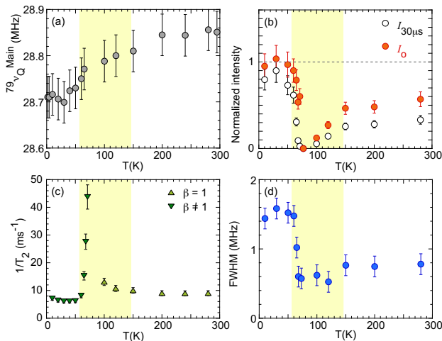
FIG. 3. (a) The main NQR peak frequency {}^{79}\nu_Q^{Main} . (b) (o) The bare integrated intensity I_{30\mu s} of the lineshapes in Fig. 2(a-b), and (●) I_0 at the limit of 2\tau = 0 , both corrected for the Boltzmann factor by multiplying temperature T . (c) 1/T_2 determined from the fit in Fig. 2(c-d) with (▲) or without (▼) fixing \beta = 1 . (d) FWHM of the {}^{79}\text{Br} NQR lineshapes. We observe only a limited number of {}^{79}\text{Br} nuclear spins due to lattice freezing in the yellow shaded region of Figs. 3 and 4.
