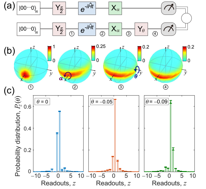
FIG. 3. Experimental procedure for extracting the FI for 19 superconducting qubits. (a) Schematic of the preparation, nonlinear evolution, optimization rotation, measurement, and comparison of the readouts of two states, with and without the collective phase pulse Y_\theta , \exp(-i\hat{J}_y\theta) , as in the Ramsey interferometer, for the extraction of the FI. (b) Experimental data of the Q functions, Q(\theta, \phi) , representing the states after ① the initial preparation, ② the nonlinear evolution with t = 48 ns, ③ the collective optimization rotation X_\alpha , \exp(-i\hat{J}_x\alpha) , with \alpha = -0.288 rad, and ④ the Ramsey pulse Y_\theta , respectively. (c) The probability distributions P_z(\theta) of the measurement observable \hat{J}_z from the single-shot readout of each qubit, for \theta = 0 rad, -0.05 rad, and -0.09 rad.
