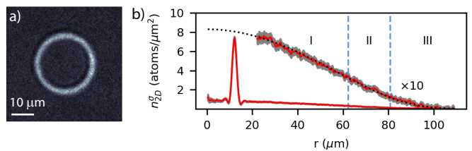
FIG. 2. a) Absorption image (10 averaged) of an equal spin mixture of {}^6\text{Li} atoms in the trap potential of Fig. 1, with 1 \times 10^4 atoms in each spin state. A magnetic field of 107.4 mT has been used to tune the scattering length to -179 \text{ nm} . The density peak is at r = 12.0(2) \text{ }\mu\text{m} . This is a 50 \times 50 \text{ }\mu\text{m} region cropped from a 215 \times 215 \text{ }\mu\text{m} image. (b) Radial column density obtained by azimuthal averaging over the full field of view. The plot is shown vertically rescaled \times 10 for r > 20 \text{ }\mu\text{m} to emphasize the broad halo extending to r = 100 \text{ }\mu\text{m} . The black dotted line is the expected density profile ( \times 10 ) for an ideal Fermi gas in our trap at T = 25 \text{ nK} . In region I the system is 3D degenerate, II is quasi-2D degenerate, and III is quasi-2D thermal. Grey band: 2\sigma variation of n_{2D}(r) when calculated separately for each image in the set.
