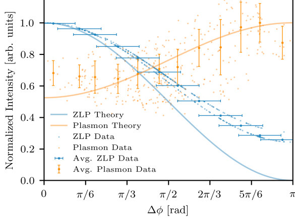
FIG. 3. Measured and modelled ZLP and plasmon intensities as a function of total relative probe phase.
