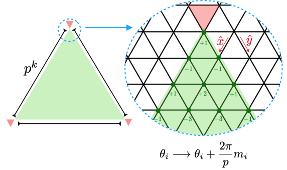
FIG. 1: The U(1) parent model (2) has a family of fractal symmetries, generated by a staggered rotation of the boson phase \theta_i \rightarrow \theta_i + \frac{2\pi}{p} m_i over a triangular region of side length which is a power of any prime number p . For each p , the fractal symmetry becomes exact for system size L^2 with L = p^k - 1 . When acting on a classical ground-state of the parent model, this transformation generates excitations at the corners of the triangular region. The action of this rotation can be visualized as Pascal’s triangle modulo p , which is a fractal with Hausdorff dimension d_H(p) = \ln(p(p+1)/2)/\ln p .
