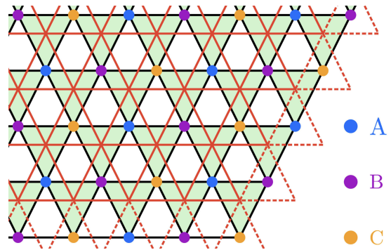
FIG. 2: The models we consider in this work involve sum of all the downward facing triangles (shaded in green); The dual of the U(1) model (Eq. 5, Eq. 15) is defined on the dual triangular lattice, whose sites are the center of each downward facing triangles of the original lattice.
