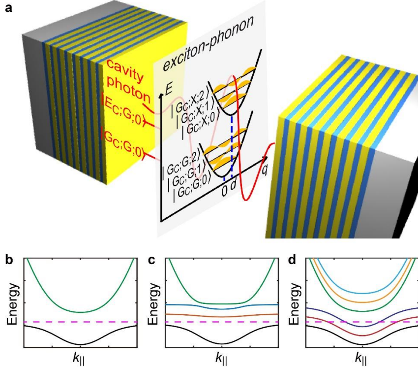
FIG. 1. (a) Schematic plot of the vibronic polariton model. (b) Simulated polariton dispersion curves under two-coupled-oscillator model. (c,d) Simulated polariton dispersion curves using vibronic polariton model under the assumption that the coupling terms with phonon-dressed photon states are deactivated (c) and activated (d). The dashed purple lines indicate the dispersion relation of the pure exciton.
