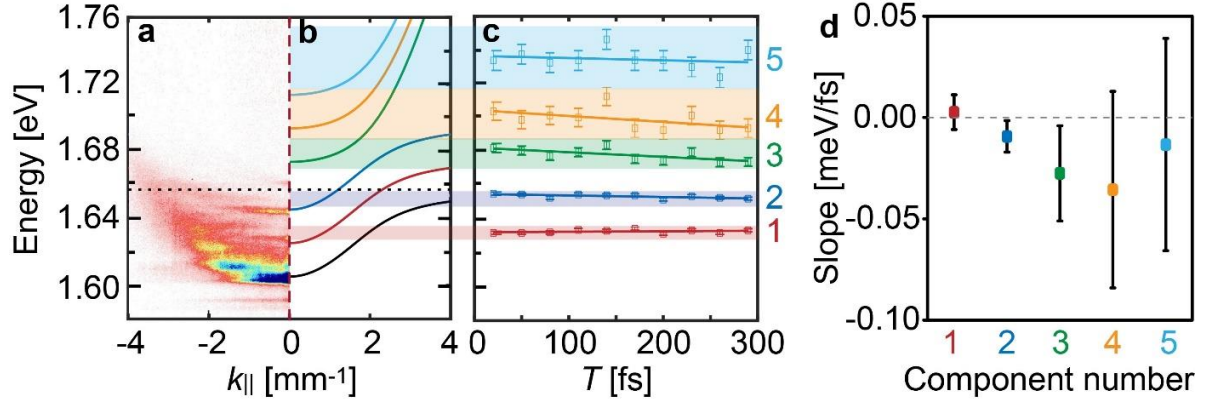
FIG. 3. (a) Energy-momentum-resolved PL map (for negative k_{||} , see Supplemental Material [20] for the full data set). (b) Simulated polariton dispersion relations using vibronic polariton model. The horizontal dotted line indicates the energy of pure excitons. (c) Retrieved energy positions (squares) of five bands as functions of T , and linear fitting results (solid lines). The error bars are evaluated as the standard deviation of the fluctuations calculated from the differences between the measured values (squares) and linear fit results (solid lines) at each T . Colored shaded areas in b and c indicate the total confidence ranges of experimentally determined energy positions from 2D spectroscopy data evaluated over all T , to facilitate comparison with the theoretical dispersion curves. (d) Linear slopes of the five fits from c, with error bars depicting 95% confidence bounds from the fit.
