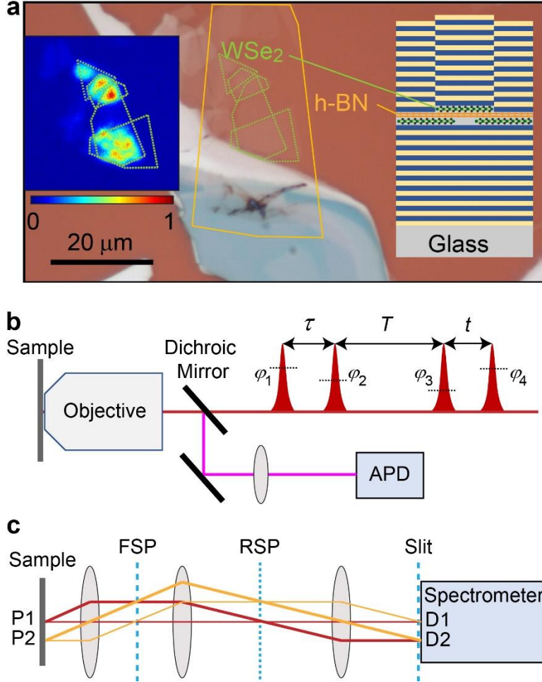
FIG. 2. (a) Microscope image of the WSe 2 /h-BN/WSe 2 structure. Insets: Map of PL intensity (left); schematic diagram of the microcavity with embedded WSe 2 /h-BN/WSe 2 heterostructure (right). (b) Schematic diagram of 2D micro-spectroscopy. (c) Detection scheme of momentum-resolved PL spectroscopy. Abbreviations: Fourier-space plane (FSP), Real-space plane (RSP), and Avalanche Photodiode (APD).
