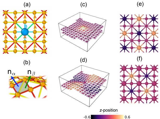
FIG. 1. (a) Square lattice model with background sites A and a single dilation site B . (b) Schematic of normals of two neighboring triangular plaquettes \alpha, \beta . (c,d) Height profiles of relaxed membranes with a single (c) positive and (d) negative dilation at T = 0 . The color represents the height relative to the zero-plane in units of the lattice spacing a_0 . The dilation nodes are indicated with a larger radius sphere. (e,f) Top views of membranes with a square array of positive (e) and negative (f) dilations in a (0, 2) array at T = 0 . Both display a checkerboard configuration characteristic of antiferromagnetism at T = 0 when spins are defined as the nodes that buckle out of plane. Node positions are visualized using OVITO software [37].
