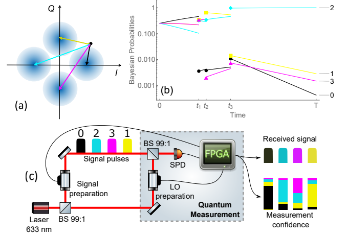
FIG. 1. (a) A constellation diagram of M = 4 coherent states that differ by phase. Fuzzy circles represent uncertainty due to shot noise. Black dot - a possible outcome of a homodyne measurement. Arrows - difference between the value obtained with a homodyne and the expected states (used in calculating \tilde{P}_C , see text); (b) an example of the experimentally measured \tilde{P}(t) in a single-shot measurement. Here, single photon detections occur three times at t_1, t_2 , and t_3 ; (c) Experimental setup. For each signal pulse, the quantum measurement determines the most likely input state and the confidence of discrimination (Bayesian probability of each of the possible states based on the measurement record, see text). The optical input for system efficiency characterization is defined at the input port of the fiber beam splitter used for displacement.
