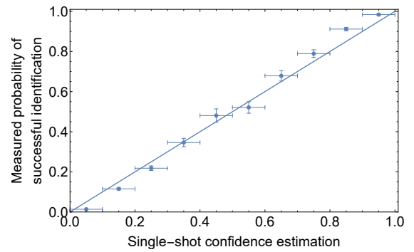
FIG. 4. Experimentally measured single shot confidence vs. the experimental ensemble average probability of a successful state discrimination obtained for faint input ( \langle n \rangle = 2.68 photons per signal pulse) prepared in one of M = 4 states. Vertical error bars correspond to one standard deviation, horizontal error bars show histogram bin size.
