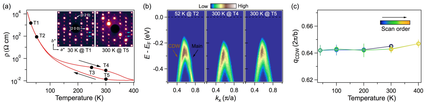
FIG. 2. Temperature evolution of lattice and electronic structures. (a) Temperature-dependent electrical resistivity with currents along the a -axis. Black arrows indicate the temperature sweep direction. Inset : electron diffractions at 30 K and 300 K. Cyan arrows indicate the CDW superlattice peaks, which, unlike the report in ref. [16], are present in both low and high resistivity states. The asymmetry of the electron diffraction pattern at 300 K is due to imperfect sample alignment relative to the incoming electron beam. (b) Photoemission intensity with 24 eV photons along \bar{\Gamma} - \bar{X} at three points along the hysteresis loop [T2, T4 and T5 in (a)]. (c) Temperature evolution of the CDW wavevector from x-ray diffraction. Error bars represent the difference in q_{\text{CDW}} as obtained from two separate CDW peaks, (0, -1 - q_{\text{CDW}}, 10) and (0, -2 + q_{\text{CDW}}, 10) .
