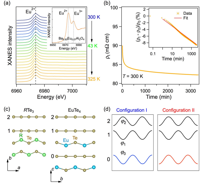
FIG. 4. Candidate mechanisms of the hysteretic transition. (a) Temperature dependence of the Eu L_3 x-ray absorption near edge structure (XANES) in \text{EuTe}_4 . Inset : XANES spectrum of \text{Ba}_{0.93}\text{Eu}_{0.07}\text{Al}_2\text{O}_4 , adapted from ref. [34]. (b) Time dependence of electrical resistivity immediately after a thermal cycle of 400 K \rightarrow 20 K \rightarrow 300 K [orange curve in Fig. S9(c)]. Inset : linear-log plot of the percentage change in resistivity relative to the first value of the time sequence ( \rho_0 ). Red line is a logarithmic fit to f(t) = A \log(t) + B , where A = -0.0215(2) and B = -0.865(5) for a time window from 1 min to 3300 min. (c) Schematic structures of R\text{Te}_3 and \text{EuTe}_4 . Due to different space groups, the out-of-plane directions have different labels by convention. (d) Illustrations of two candidate out-of-plane CDW configurations in \text{EuTe}_4 . The relative CDW phase between Te monolayer and Te bilayer ( \phi \equiv \varphi_1 - \varphi_0 ) is assigned to 0 (I) or \pi (II).
