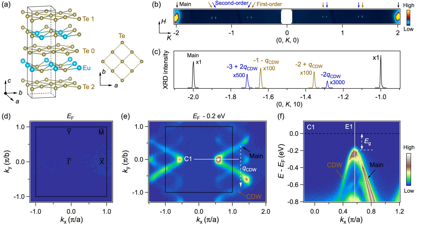
FIG. 1. Incommensurate CDW in \text{EuTe}_4 . (a) Crystal structure of \text{EuTe}_4 . Black lines denote the primary unit cell, which contains two motifs of the Te square lattice ( right panel ): bilayer (Te 1 and Te 2) and monolayer (Te 0). (b) Room temperature x-ray diffraction pattern taken with 30.6 keV photon energy in transmission mode. (c) Room temperature high-resolution x-ray intensity cut along the (0, K, 10) direction, taken with 11 keV photons in reflection geometry. (d) Room temperature Fermi surface map, showing no intensity contrast. (e) ARPES constant energy contour at 0.2 eV below the E_F , measured at T = 20 K. (f) Band dispersions at 55 K, corresponding to the C1 cut. Photon energy used was 90 eV in (d)(e) or 24 eV in (f).
