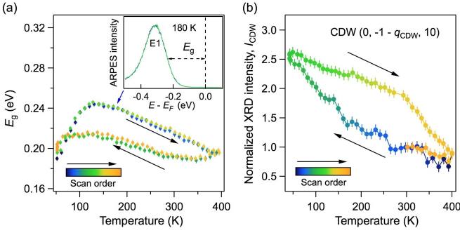
FIG. 3. Giant thermal hysteresis within the CDW state. (a) Leading edge gap E_g from two thermal cycles 50 K \rightarrow 400 K \rightarrow 50 K \rightarrow 400 K \rightarrow 50 K. E_g is taken at its maximum value at momentum E1 [see Fig. 1(f)]. The turn around 120 K is interpreted as a change in the chemical potential. Inset : two representative energy distribution curves at E1, measured at 180 K in two successive heating branches. (b) Temperature dependence of integrated intensity of a first-order CDW peak, normalized by its value at 300 K at the end of a 400 K \rightarrow 42 K \rightarrow 400 K \rightarrow 300 K sequence. The error bars in (a) and (b) represent the statistical uncertainty derived from the fitting procedure and the maximum difference between the two cooling branches from 400 K to 300 K, respectively. See Ref. [18] for raw data.
