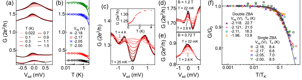
FIG. 4. Temperature dependence of single- and double-peak zero bias anomalies. (a) Temperature dependence of four different single-peak ZBAs ( B = 0 ). (b) Peak height of ZBAs in (a) as a function of T , measured at V_{sd} = 0 . Solid lines are fits to the data using Eq. 1, with T_K as the fitting parameter. From top-to-bottom T_K = 8.5, 7.0, 6.6 , and 8.4 K. (c) Temperature dependence of the double-peak ZBA at B = 0 . The inset shows G against T at V_{sd} = 0 . (d) and (e) Temperature dependence of two double-peak ZBAs at B_{||} = 1.2 T and 0.72 T, respectively. The values of B_{||} are those where the peaks merge into a single peak. (f) Normalized ZBA peak height ( G/G_0 ) at V_{sd} = 0 for both the single- and double-peak ZBAs. For each data set G_0 is the ZBA peak height at base temperature and V_{sd} = 0 . The black line is plotted using the Anderson model for a Kondo impurity, Eq. 1.
