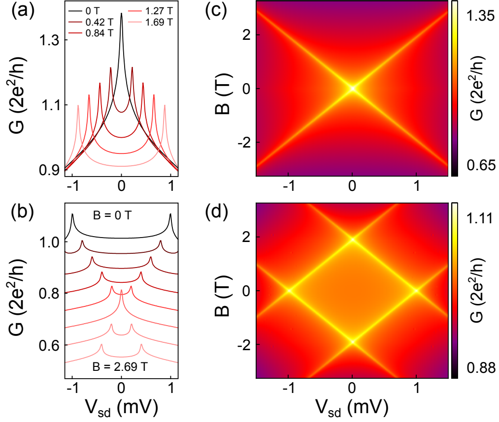
FIG. 3. Theoretical simulation of the differential conductance using a quantum master equation approach. (a) and (b) G against V_{sd} in the absence and presence of Rashba SO coupling, respectively, for selected B . Data in (b) are offset vertically from B = 0 (top trace) in increments of -0.06 \times 2e^2/h , for clarity. Data in (a) are not offset. (c) and (d) Corresponding colormaps of G as a function of B and V_{sd} without and with SO coupling, respectively.
