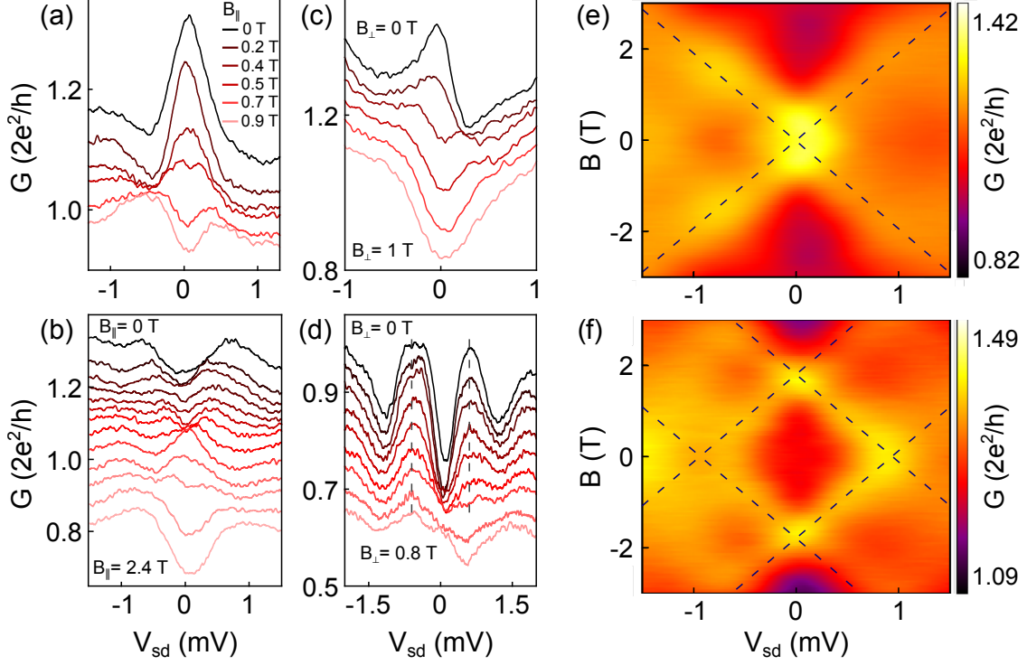
FIG. 2. Magnetic-field dependence of the single- and double-peak zero-bias anomalies. (a) and (b) G as a function of V_{sd} for single- and double-peak ZBAs, respectively. The external magnetic field is applied parallel ( B_{\parallel} ) to B_{SO} and stepped between traces. (c) and (d) Same as (a) and (b) but for the external magnetic field applied perpendicular ( B_{\perp} ) to B_{SO} . In (a)–(d) data are offset vertically for clarity. (e) and (f) Colormaps of G as a function of B_{\parallel} and V_{sd} , for the single- and double-peak ZBA, respectively. The position of ZBA peaks are well described by dashed lines eV_{sd} = \pm g\mu_B(B_{\parallel} + B_{SO}) , for (e) B_{SO} = 0 and (f) B_{SO} = \pm 1.8 T. B_{SO} in (f) differs from the estimate for Fig. 2(d) since data are measured at different V_{sg} and G . All data are obtained at T = 22 mK.
