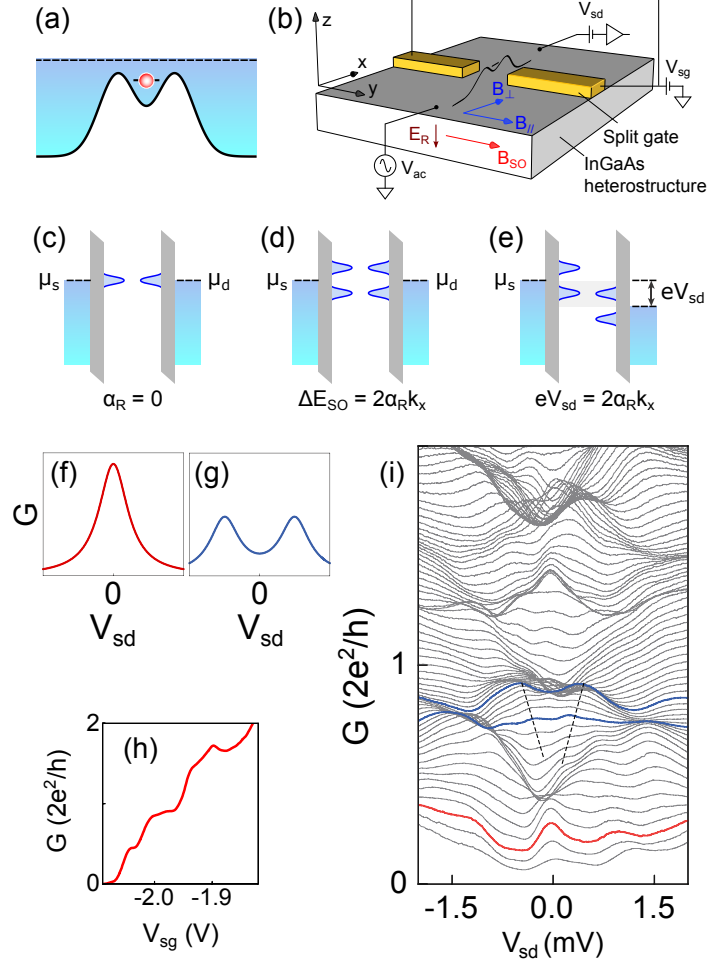
FIG. 1. Illustrations of the Kondo and spin-orbit coupled system, and zero-bias anomalies. (a) Schematic profile of the bound-state potential in the QPC. (b) Simplified circuit schematic. E_R and B_{SO} indicate directions of the electric field from the structural inversion asymmetry and the effective magnetic field due to SO coupling, respectively. (c)–(e) Energy-level diagrams of a Kondo impurity coupled to source and drain leads at three situations described in the main text. (f) and (g) Sketches of G against V_{sd} in the absence and presence of SO coupling, respectively. (h) QPC conductance at V_{sd} = 0 . Plateaus are slightly suppressed below expected values due to imperfect transmission through the QPC. (i) QPC conductance as a function of V_{sd} , with V_{sg} stepped incrementally between traces.
