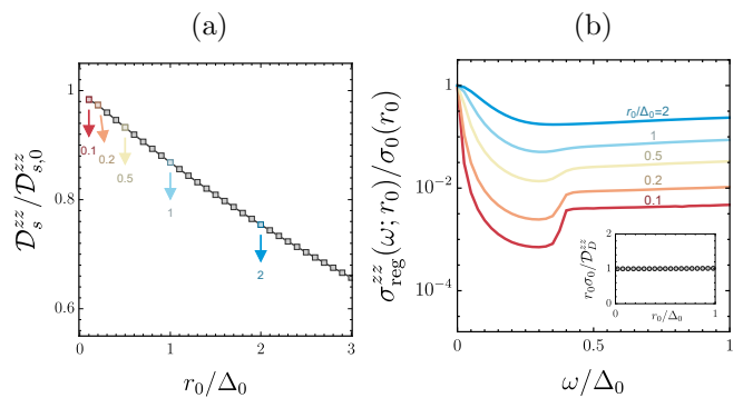
FIG. 2. (a) The r_0 dependence of the superfluid weight, \mathcal{D}_s^{zz}(r_0) . The clean limit of supercurrent is interpolated as a positive value, \mathcal{D}_{s,0}^{zz} = 0.163e^2\sqrt{m\mu^3}/\hbar^3 . (b) The frequency and r_0 dependence of regular part of conductivity, \sigma_{\text{reg}}^{zz}(\omega; r_0) . The different values of r_0/\Delta_0 = \{0.1, 0.2, 0.5, 1, 2\} are used and denoted with different colors. Inset shows \sigma_0^{zz}(r_0) = \mathcal{D}_D^{zz}/r_0 in the small r_0 limit with a Drude-weight, \mathcal{D}_D^{zz} = 0.168e^2\sqrt{m\mu^3}/\hbar^3 .
