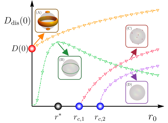
FIG. 1. Schematic DOS plot at zero energy ( D_{\text{dis}}(0) ) with various nodal superconductors as a function of impurity strength , r_0 = n_{\text{imp}} V_0^2 . The insets show zero-energy excitations in the momentum space of four different states, BG-FS (A), line-nodal (B), point-nodal (C) and fully gapped (D) superconductors. The linear dependence of DOS on r_0 is a distinctive property of a BG-FS. Here, r^* is a resonant impurity strength for a line-nodal superconductor [53] and (r_{c,1}, r_{c,2}) are critical values of r_0 for point-nodal and fully gapped superconductors, respectively (See SM). The functional forms of \delta D_{\text{dis}}(0; r_0) = D_{\text{dis}}(0; r_0) - D(0) are tabulated in Table I.
