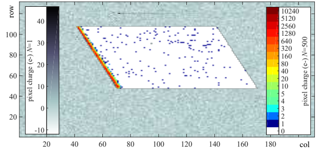
FIG. 6: Experiment combining ROI and EOI. Two color scales: on the left pixels with N = 1 and a noise of 3\text{ e}^- , and on the right pixels with N = 500 and a readout noise of 0.13\text{ e}^- (and therefore quantized charge).
