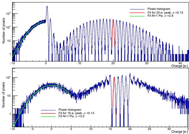
FIG. 5: Pixel histograms for EOI technique. N = 500 for charge ranges 0\text{ e}^- to 42\text{ e}^- (top) and 15\text{ e}^- to 19\text{ e}^- (bottom).
