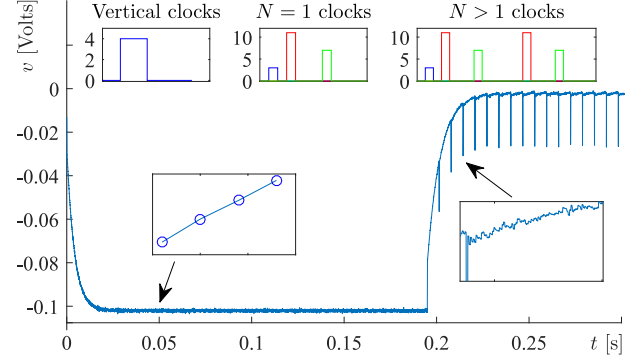
FIG. 2: Baseline of raw video signal in volts. Part of one row, the first 3039 pixels use N = 1 and the others N = 100 . At the top, insets illustrate clock sequences and their voltage swings. At the bottom, zoomed regions of the baseline corresponding to the samples of a single pixel read with N = 1 at t \approx 0.05 and with N = 100 at t \approx 0.215 .
