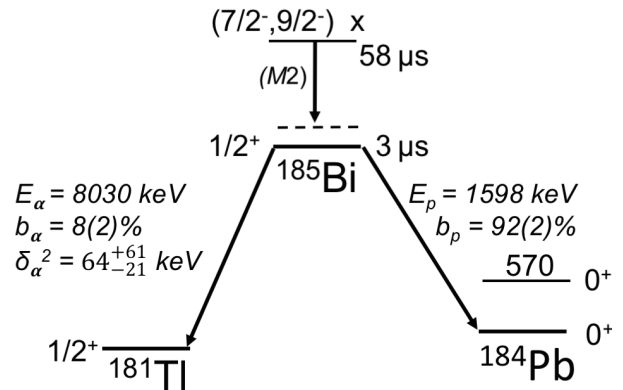
FIG. 4: The proposed decay pattern of ^{185}\text{Bi} . The excitation energy of the 58- \mu s isomeric state is not yet known. The most likely spin-parity assignment is 7/2^- or 9/2^- , with different decay paths towards the 3- \mu s 1/2^+ gs, depending on the specific assignment, see text for details. The nature of the intermediate level(s), shown with a dashed line, is discussed in the text. The branching ratios, b_p and b_\alpha , are determined in the present work and the energy of the excited state in ^{184}\text{Pb} is given in keV.
