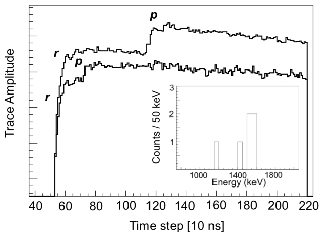
FIG. 3: Example waveforms for recoil ( r ) - proton ( p ) decay events, where the recoil is followed by a ^{184}\text{Pb} \alpha decay in the same DSSD pixel. The inset shows the energy spectrum obtained by extracting the proton-decay energies from the six pile-up waveforms. A matrix of ^{185}\text{Bi}(p)\text{-}^{184}\text{Pb}(\alpha) decay events is shown in Fig. 4 of the SM.
