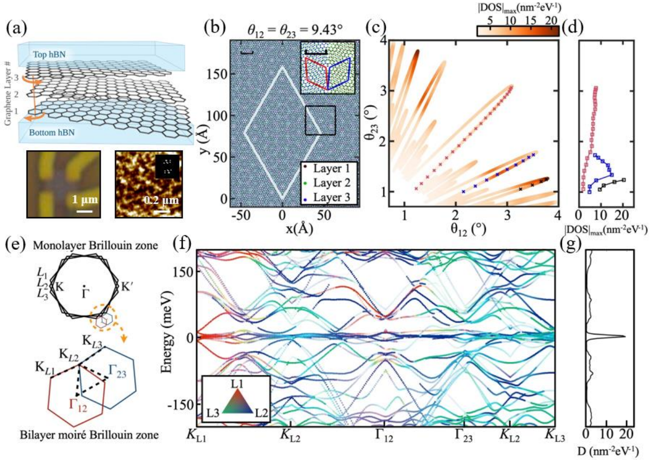
Figure 1. Moiré of Moiré (MoM) Superlattices in Twisted Trilayer Graphene (tTLG). (a) Schematic of the hBN-encapsulated tTLG device, consisting of three monolayer graphene consecutively twisted with respect to the previous layer. (Bottom-left) Optical microscope image of a typical device under study. (Bottom-right) AFM topology of tTLG on hBN, made at consecutive twist angles of 1.64^\circ for demonstration of tTLG MoM. Irregular and triangular-like patterns with length scale on the order of 300 nm are barely visible, suggesting a plethora of coexisting MoM length scales accompanying the dominating MoM lattice. Inset: Dominating Fourier components in the FFT spectrum, corresponding to length scales of 120 ~ 260 nm, which qualitatively agrees with experimental design. (b) Atomic positions in tTLG at a set of commensurate angles \theta_{12} = \theta_{23} = 9.43^\circ demonstrating the MoM superlattice. White parallelogram: MoM supercell. (Inset) Zoom-in of the area inside the black box showing the bilayer moiré pattern. The left (right) shows only layers 2 and 1 (3), the red (blue) parallelograms show the corresponding bilayer moiré supercells. Both scale bars are 10 Å. (c) Possible twist angle combinations for MoM area A_1 = 6438 \text{ nm}^2 (MOM-1). Color scale represents the density of state maximum. (d) 1D cuts along twist angle configurations near \theta_{12} = \theta_{23} , \theta_{12} = 2\theta_{23} and \theta_{12} = 3\theta_{23} , respectively. (e) Monolayer Brillouin zone of the three individual layers (top) and the bilayer moiré Brillouin zone formed between adjacent bilayer pairs (bottom). (f) Band structure at \theta_{12} = 2.9^\circ , \theta_{23} = 1.4^\circ along the high symmetry line indicated by the dashed line in (e). Colors indicate the projected weight onto the state at the center momentum in each layer. Red: layer 1; blue: layer 2; green: layer 3. (g) Normalized density of states corresponding to band structure shown in (f), with zero-energy peak value comparable to that of tBLG.
