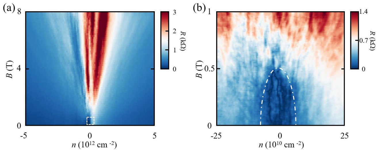
Figure 4. Magneto-Transport at Larger Carrier Density Span. (a) Resistance of MoM-1 as a function of magnetic field and a large range of carrier density. Zero resistance states are only observed in a very small density range near zero carrier density. (b) Magneto-transport data in a smaller range of carrier density, displaying a very complicated Hofstadter butterfly pattern, in which zero resistance states exist up to \sim 500 mT.
