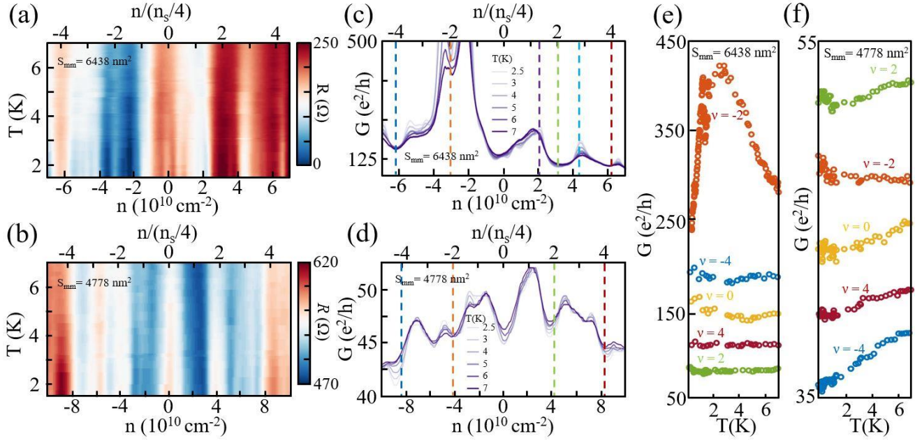
Figure 2. Insulating and Semi-metallic Behavior at \nu = \text{even Integer Fillings} of Two MoM Superlattices. (a) Measured 4-probe resistance of MoM-1 (unit cell size = 6438 \text{ nm}^2 ) and (b) MoM-2 (unit cell size A_2 = 4778 \text{ nm}^2 ) as a function of temperature and carrier density n . Resistance peaks are observed at all \nu = n/(n_s/4) = \text{even integer fillings} , where n_s is the carrier density corresponding to four charge carriers per MoM unit cell. (c) Line traces of four-probe conductance as a function of carrier density taken at different temperatures of MoM-1 and (d) MoM-2. (e) Conductance as a function of temperature at each even filling for MoM-1 and (f) MoM-2. Data are offset to separate each curve.
