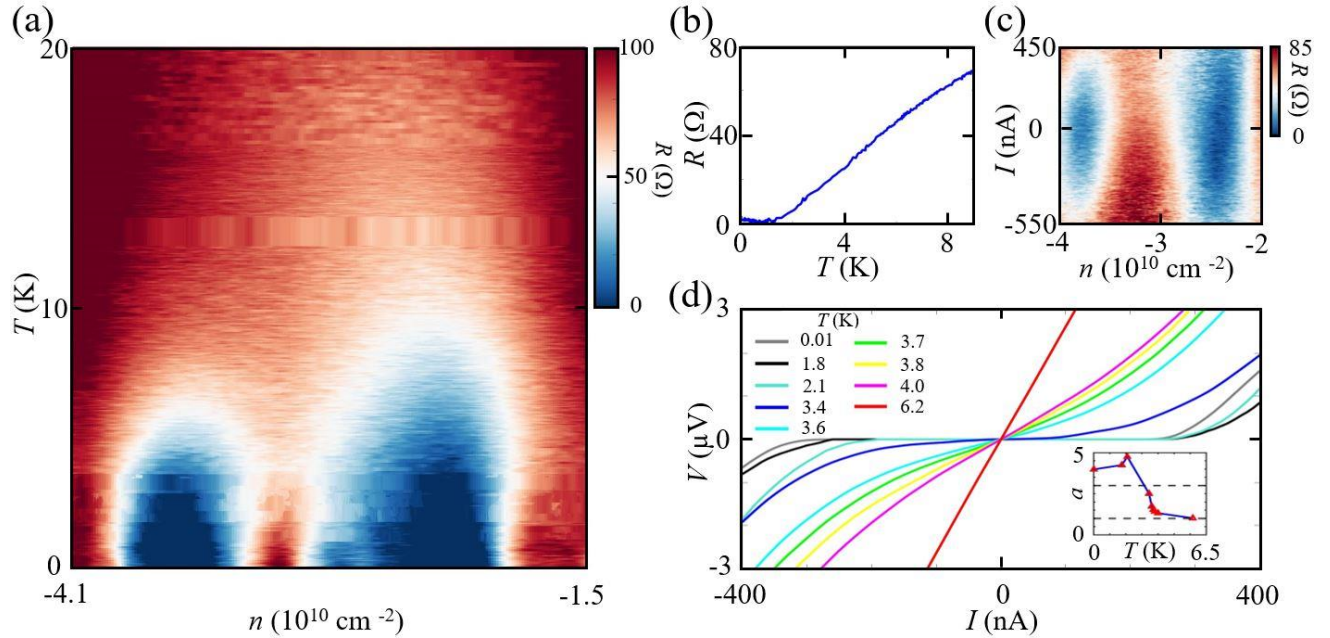
Figure 3. Temperature and Bias Characteristics of Superconducting-like States. (a) Measured 4-probe resistance of MoM-1 as a function of carrier density and temperature. At half-filling of the MoM superlattice ( n \sim -3.22 \times 10^{10} \text{ cm}^{-2} ), correlated insulating behavior is observed with two adjacent zero-resistance domes. (b) Differential resistance as a function of temperature near the center of the right zero-resistance dome. (c) Differential resistance as a function of carrier density and DC bias offset at 3 K. Zero resistance states symmetric with respect to zero bias exist up to J_c \sim 200 nA. (d) I - V characteristics at different temperatures, near the center of the right zero-resistance dome. The I - V curve power law exponent goes from 1 to 3 as temperature decreases, consistent with the BKT model for a typical 2D superconductor. (Inset) The temperature dependence of the power law exponent \alpha , from which a critical temperature T_{\text{BKT}} \sim 3.4 K is extracted.
