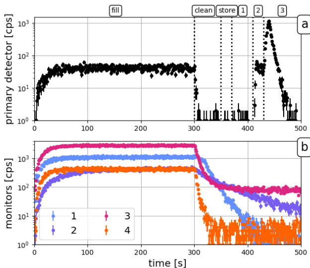
FIG. 2. a) Primary detector coincidence counts from analysis A for a typical t_{\text{store}} = 20 s run cycle. From left to right, the dotted vertical lines mark the time windows for filling, cleaning, storing, and three counting stages. b) The count rate during the run cycle for the monitors deployed in the 2018 analysis.
