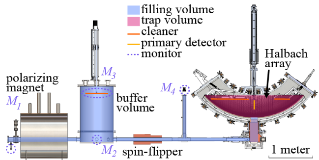
FIG. 1. The UCN \tau apparatus configuration for the 2018 campaign, with the volumes occupied by UCN, cleaner surfaces, primary detector, and monitors highlighted. The polarizing magnet selects the high-field-seeking UCN. UCN are then “pre-cleaned” in the buffer volume, spin-flipped to the trappable low-field-seeking spin state, and loaded into the trap. The 2017 configuration was the same as that of Ref. [30].
