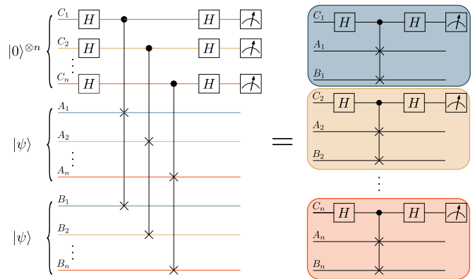
FIG. 1. Circuit for the n -qubit parallelized SWAP test. Given two copies of the quantum state |\psi\rangle , and n ancilla qubits, the n -qubit parallelized SWAP test consists of employing the k -th ancilla to perform a controlled swap test on the k -th qubit of each copy of |\psi\rangle . Since the n SWAP test can be factorized, one can perform them in parallel, leading to a constant depth circuit.
