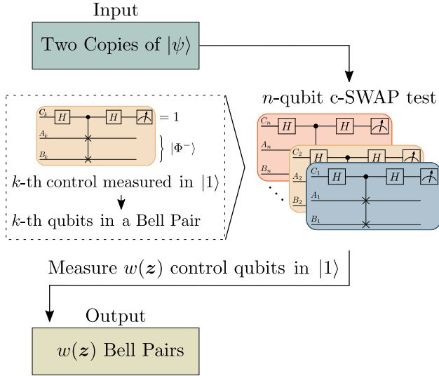
FIG. 2. Protocol for concentrating entanglement. Given two copies of |\psi\rangle , one can employ the n -qubit parallelized SWAP test to prepare Bell pairs between qubits in the different copies of |\psi\rangle . Specifically, measuring the k -th control qubit in the state |1\rangle implies that the joint state of the k -th qubit of each copy of |\psi\rangle is the Bell state |\Phi^-\rangle = \frac{1}{\sqrt{2}}(|01\rangle - |10\rangle) . Hence, a single run of the n -qubit parallelized SWAP test has a probability p(\mathbf{z}) of concentrating the multipartite entanglement in the copies of |\psi\rangle and producing w(\mathbf{z}) Bell pairs.
