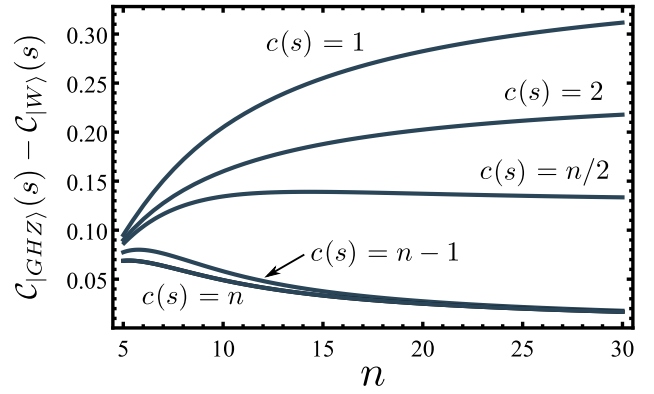
FIG. 3. Comparison of the Concentratable Entanglements for GHZ and W states. In the figure we show the difference C_{|GHZ\rangle}(s) - C_{|W\rangle}(s) versus the number of qubits n for different sets s with cardinalities c(s) = 1, 2, n/2, n-1, n . In all cases we find C_{|GHZ\rangle}(s) > C_{|W\rangle}(s) .
