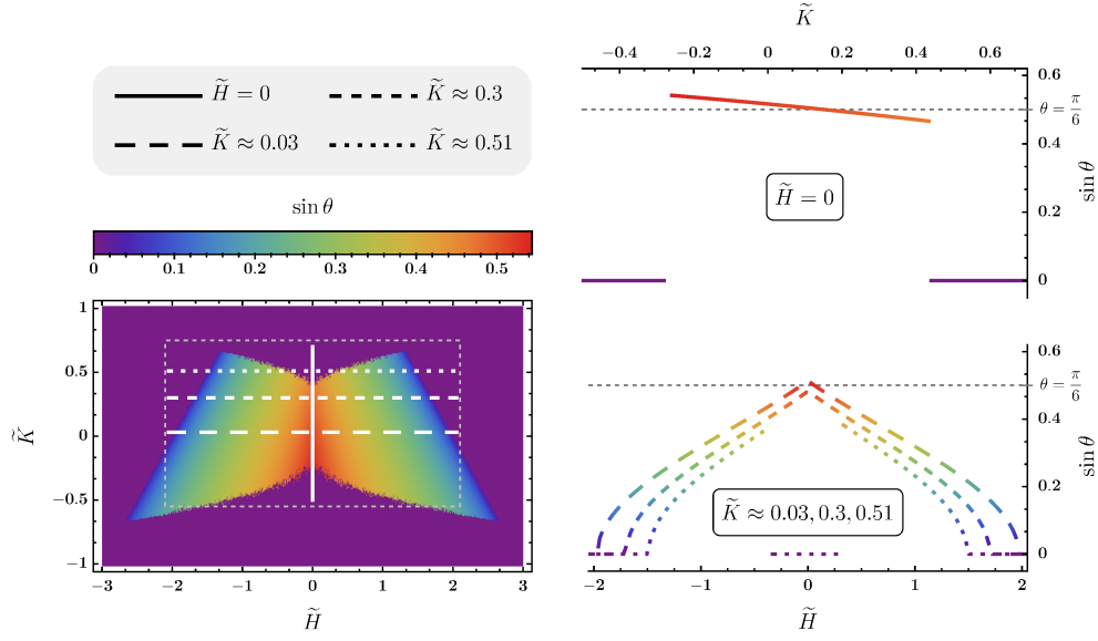
FIG. 2: The color plot is obtained by numerical minimization of the function \mathcal{E}(\mathbf{k}, \mathbf{n}, \theta) of Eq. (6) and represents the value of \sin \theta (the span of magnetic cone) at the global minimum, provided external magnetic field is directed as \tilde{\mathbf{H}} = \tilde{H}(0, 1, 1)/\sqrt{2} . Non-collinear magnetic cone state (finite \theta and \mathbf{k} ) is realized for moderate values of \tilde{K} and \tilde{H} . The upper left panel shows the horizontal crosssection with \tilde{H} = 0 , while the lower left panel shows three vertical crosssections for \tilde{K} = 0.03, 0.3 , and 0.51 . The angle \theta smoothly deviates from zero across the lines \tilde{K} = 2 - |\tilde{H}| , which correspond to the second order phase transition. Noisy borders for \tilde{K} \approx \pm 0.5 correspond to the first order phase transition from collinear to a non-collinear state with a finite \theta . The corresponding jumps are also seen in the left panels.
