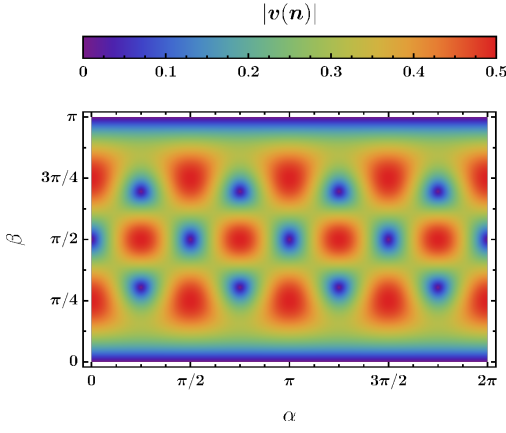
FIG. 3: Absolute value of the vector \mathbf{v} that defines the asymmetry of the magnon dispersion \delta\omega_{\mathbf{q}} = -16B\mathbf{v} \cdot \mathbf{q} as the function of the magnetization direction \mathbf{n} = (\cos \alpha \sin \beta, \sin \alpha \sin \beta, \cos \beta) .
