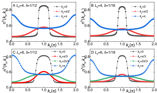
FIG. 5. (Color online) Hole momentum distribution function n^h(k_x, k_y) for L_y = 4 cylinders at (A) \delta = 1/12 and (B) \delta = 1/16 , and L_y = 6 cylinders at (C) \delta = 1/12 and (D) \delta = 1/18 at different k_y as a function of k_x in unit of \pi .
