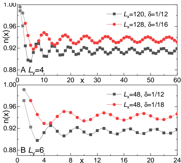
FIG. 2. (Color online) Charge density profiles n(x) for (A) L_y = 4 cylinders at \delta = 1/12 and \delta = 1/16 , and (B) L_y = 6 cylinders at \delta = 1/12 and \delta = 1/18 . The exponent K_c is extracted using Eq. (3), with the data points in grey neglected to minimize boundary effects.
