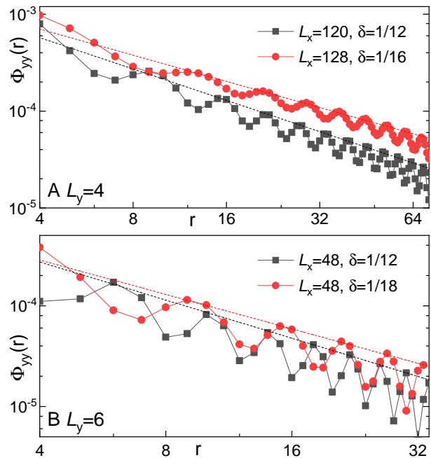
FIG. 1. (Color online) Superconducting pair-field correlations \Phi_{yy}(r) on double-logarithmic scales for (A) L_y = 4 cylinders at \delta = 1/12 and \delta = 1/16 , and (B) L_y = 6 cylinders at \delta = 1/12 and \delta = 1/18 . r is the distance between two Cooper pairs in the \hat{x} direction. The dashed lines denote power-law fitting to \Phi_{yy}(r) \sim r^{-K_{sc}} .
