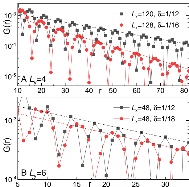
FIG. 4. (Color online) Single-particle Green function G(r) for (A) L_y = 4 cylinders at \delta = 1/12 and \delta = 1/16 , and (B) L_y = 6 cylinders at \delta = 1/12 and \delta = 1/18 on the semi-logarithmic scale. Dashed line denote exponential fitting G(r) \sim e^{-r/\xi_G} where r is the distance between two sites in the \hat{x} direction.
