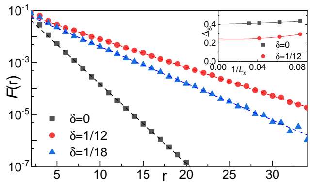
FIG. 3. (Color online) Spin-spin correlations F(r) for L_y = 6 cylinders at \delta = 0 , \delta = 1/12 and \delta = 1/18 on the semi-logarithmic scale. Dashed lines denote exponential fit F(r) \sim e^{-r/\xi_s} , where r is the distance between two sites in the \hat{x} direction. Inset: Spin gap \Delta_s for L_y = 6 cylinders at \delta = 0 and \delta = 1/12 . Solid lines denote second-order polynomial fitting.
