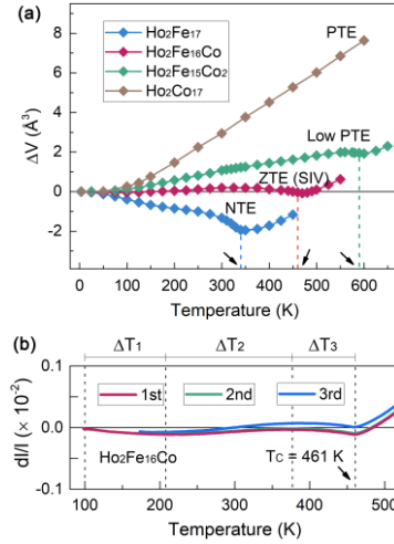
FIG. 2. (a) Temperature dependence of relative unit cell volume determined by NPD refinements from 3 to 650 K for \text{Ho}_2(\text{Fe},\text{Co})_{17} compounds; (b) Apparent zero thermal expansion of \text{Ho}_2\text{Fe}_{16}\text{Co} compound determined by thermal dilatometer from 100 to 520 K. The coefficients of thermal expansion are further determined within three temperature windows (calculated by using the first measurement): \bar{\alpha}_l = -0.8(1) \times 10^{-6} \text{ K}^{-1} , \Delta T_1 = 100\text{-}208 \text{ K} ; \bar{\alpha}_l = 0.6(0) \times 10^{-6} \text{ K}^{-1} , \Delta T_2 = 208\text{-}377 \text{ K} ; \bar{\alpha}_l = -0.9(1) \times 10^{-6} \text{ K}^{-1} , \Delta T_3 = 377\text{-}461 \text{ K} , respectively.
