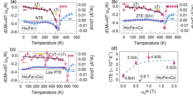
FIG. 5. (a) The rates of the change of |\Sigma M_{\text{Fe}}| ( d|\Sigma M_{\text{Fe}}|/dT ) and unit cell volume ( dV_{\text{obs}}/dT ) as a function of temperature in \text{Ho}_2\text{Fe}_{17} , (b) \text{Ho}_2\text{Fe}_{16}\text{Co} and (c) \text{Ho}_2\text{Fe}_{15}\text{Co}_2 compounds, respectively; (d) The coefficients of thermal expansion (CTEs, 5-250 K) as a function of applied magnetic field from 0 to 2 T for \text{Ho}_2\text{Fe}_{16}\text{Co} compound.
