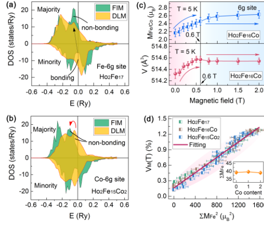
FIG. 3. (a) Atomic resolved contribution to density of state (DOS) of Fe atoms at 6g site for \text{Ho}_2\text{Fe}_{17} compound; (b) Atomic resolved contribution to the DOS of Co atoms at 6g sites for \text{Ho}_2\text{Fe}_{15}\text{Co}_2 compound; (c) Magnetic moments of Fe/Co atoms ( M_{\text{Fe/Co}} ) at 6g site and unit cell volume as a function of applied magnetic field for \text{Ho}_2\text{Fe}_{16}\text{Co} compound at 5 K; (d) Positive correlation between the magnetic moments of Fe-sublattice ( |\Sigma M_{\text{Fe}}| ) and the contribution of magnetic ordering to the unit cell volume ( V_M(T) ). The inset shows the |\Sigma M_{\text{Fe}}| as a function of Co content.
