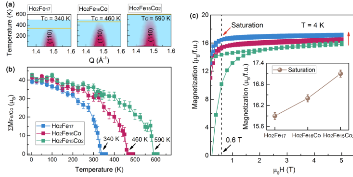
FIG. 1. (a) Contour plot of the neutron powder diffraction (NPD) intensity of magnetic peaks (110) for the three investigated samples: \text{Ho}_2\text{Fe}_{17} , \text{Ho}_2\text{Fe}_{16}\text{Co} and \text{Ho}_2\text{Fe}_{15}\text{Co}_2 . Yellow line indicates the Curie temperature ( T_C ); (b) Temperature dependence of magnetic moments of Fe/Co-sublattice ( \Sigma M_{\text{Fe/Co}} ) determined by NPD refinements; (c) Magnetization as a function of applied magnetic field (up to 50 kOe) at 4 K for \text{Ho}_2\text{Fe}_{17} , \text{Ho}_2\text{Fe}_{16}\text{Co} and \text{Ho}_2\text{Fe}_{15}\text{Co}_2 , respectively. The inset shows the saturation magnetization for these three samples.
