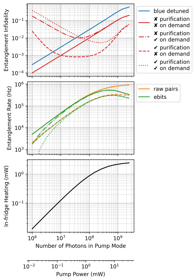
FIG. 2. In the top figure we see the infidelity of the obtained microwave Bell pair in different regimes. The blue-detuned “squeezing” implementation has higher infidelity due to populating higher-than-one-photon states (blue line). The red-detuned “beam splitter” implementation requires preparing the microwave resonator in the |1\rangle state but does not suffer from the aforementioned excitations. We further investigate the red-detuned approach followed by purification and/or storage for on-demand use (red lines). Besides the \sim \frac{g}{\gamma} infidelity in the solid lines, we see that storage at low generation rates causes an infidelity floor, due to finite microwave lifetime. The middle figure takes all red-detuned regimes from the top plot and presents their rates of entanglement generation (orange lines) and rate of equivalent ebit generation, i.e., the hashing yield [44] (green lines). The bottom figure gives the in-fridge heating due to the intrinsic loss of the optical resonator. Evaluated at g_0 = 1 \text{kHz} , \gamma_e = \gamma_i = 100 \text{MHz} , microwave loss \gamma_{\text{MW}} = 1 \text{kHz} , pump wavelength \lambda_p = 1500 \text{nm} , microwave gate fidelity 0.999, and microwave resonator reset time of 1 \mu\text{s} (state of the art values [17, 32, 43]).
