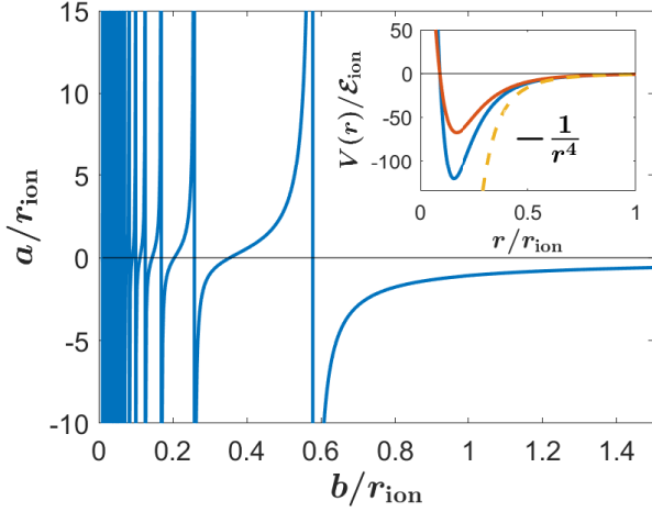
FIG. 1. The atom-ion s -wave scattering length a as a function of b . The inset shows the atom-ion potential for b/r_{\text{ion}} = 0.3 and 0.35 .
