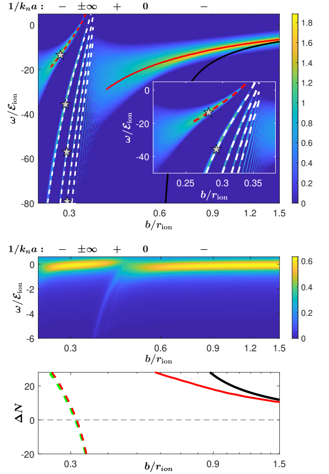
FIG. 2. The zero momentum ion spectral function A(\omega) as function of the potential parameter b and the corresponding scattering length a for n_0 r_{\text{ion}}^3 = 1 (top) and n_0 r_{\text{ion}}^3 = 0.01 (middle). The black line is the mean-field energy, the red line is the ladder approximation for the attractive polaron present for b/r_{\text{ion}} \gtrsim 0.5 , the red dashed line the repulsive polaron present for b/r_{\text{ion}} \lesssim 0.34 , and the white lines are the molecular states obtained from the Bethe-Salpeter equation. The stars \star signify the breakdown of the Bogoliubov approximation. (bottom) The number of atoms in the dressing cloud with the same color coding as the top panel, except the white molecular lines, which are represented as green lines. In the top panel, we take the logarithm to the spectral function, which visually makes the width appear larger. The middle panel is in linear scale.
