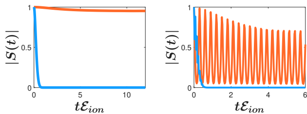
FIG. 3. In the left panel |S(t)| is shown for b/r_{\text{ion}} = 2 (orange) and b/r_{\text{ion}} = 0.5 (blue). The right panel shows |S(t)| for b/r_{\text{ion}} = 0.3 (orange) and b/r_{\text{ion}} = 0.25 (blue). We take n_0 r_{\text{ion}}^3 = 1 .
