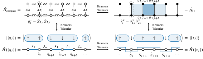
FIG. 1. Schematic depiction of the model and its mapping to a bond-disordered transverse field Ising model. A Kramers–Wannier duality of the compass model (1) along the rungs isolates the conserved charges \hat{q}_i^z = \hat{Z}_{1,i} \hat{Z}_{2,i} . Within each charge sector, specified by the configuration \{q_j\} , the Hamiltonian of the \hat{\eta} spins \hat{H}(\{q_j\}) corresponds to an Ising model with nearest neighbour coupling J_{i,i+1} = \Gamma_1 + \Gamma_2 q_i q_{i+1} .
