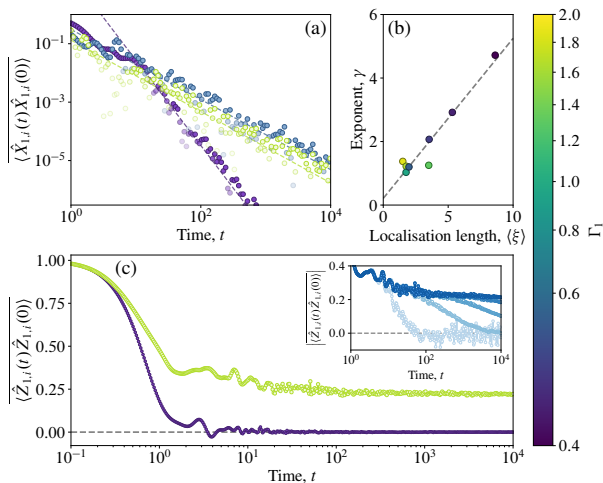
FIG. 3. Time dependence of the diagonal elements of the infinite-temperature dynamical structure factor in the compass spins, \hat{X}_{\alpha,j} and \hat{Z}_{\alpha,j} , for L = 48 ( N = 96 spins), and \Gamma_2 = \Delta = 1 . (a) The XX correlator exhibits a decay consistent with Eq. (9): Power law \sim t^{-\gamma} , with an exponent proportional to the localisation length \xi , as shown in panel (b). Conversely, the ZZ correlator (c) is diagonal in the conserved charges \{\hat{q}_j^z\} , and hence maps directly onto the corresponding spin correlation function of the disordered TFIM (2). The inset shows the divergence of the time scale over which the plateau decays with system size in the ferromagnetic phase (shown for L = 8, 16, 24, 32, 40 ).
