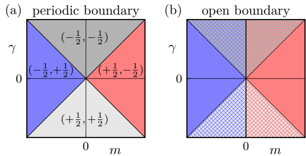
Figure 1. Topological phase diagram of one-dimensional non-Hermitian Dirac fermions with particle-hole symmetry and chiral symmetry. (a) Periodic boundary conditions. A pair of half-integer winding numbers ( \nu_+, \nu_- ) distinguishes four phases: Two Hermitian (red and blue) and two genuinely non-Hermitian phases (grey), separated by lines \gamma = \pm m . (b) Open boundary conditions. The line m = 0 separates phases with a different number of zero energy boundary eigenstates. For the boundary conditions (3), a positive mass implies the existence of a boundary state at each end (red), which are absent for a negative mass (blue). The lines \gamma = \pm m now indicate that the bulk (and boundary) Green function change from exponential decay to exponential growth.
