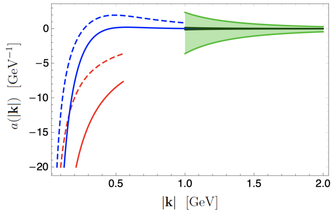
FIG. 3: Integrand functions defined in Eq. (11), appearing in the matching relations (9) and (10) for the LNV coupling \tilde{\mathcal{C}}_1 : a_\chi(|\mathbf{k}|) (solid red line extending to |\mathbf{k}| = 4m_\pi ), a_{<}(|\mathbf{k}|) (solid blue line), and a_{>}(|\mathbf{k}|) (dark-green thin band obtained by taking the range \bar{g}_1^{NN} \in [-10, 10] ). The dashed red/blue lines and light green band correspond to the integrands a_{\chi, <, >}(|\mathbf{k}|) entering the matching relation for the CIB coupling \tilde{\mathcal{C}}_1 + \tilde{\mathcal{C}}_2 . The light green band corresponds to the range \bar{g}_{LR}^{NN} \in [-10, 10] .
