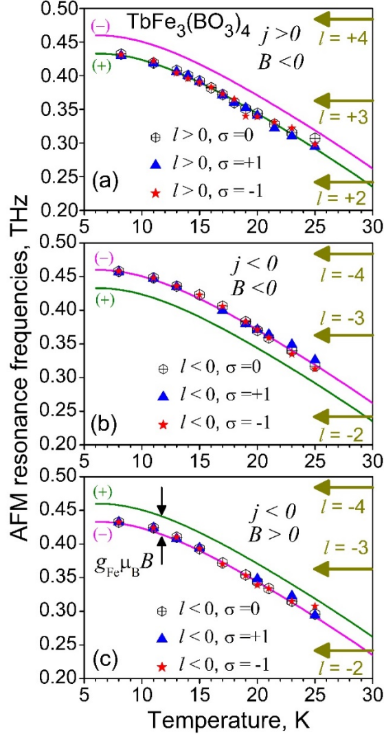
FIG. 4. (color online) Total angular momentum dichroism in Tb-FB revealed in the temperature dependencies of the AFM resonance frequencies \hbar\Omega_M^\pm(B, T) for different combinations of the \vec{B} direction and the sign of j for the vortex beams. (a) j > 0 , B < 0 , (b) j < 0 , B < 0 , and (c) j < 0 , B > 0 . Solid curves correspond to the AFM frequencies \hbar\Omega_M^\pm(B, T) measured using conventional circularly polarized light. The color code for the curves (olive and magenta) is the same as for \hbar\Omega_M^\pm(B) lines in FIG. 1(e). The measurement geometry is the same as shown in FIG. 2(c) but with various input polarizations \vec{e}_y for black, \vec{e}_L for blue, and \vec{e}_R for red symbols.
