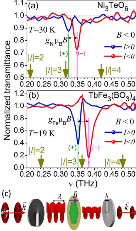
FIG. 2 (color online) Vortex dichroism for higher orders of the OAM for (a) NTO at T=30 K and (b) Tb-FB at T=19 K. Normalized transmittance spectra for two linearly polarized LG vortex beams \vec{e}_{l>0} (blue spectra) and \vec{e}_{l<0} (red spectra) were taken at B = -0.47 T that brings the AFM resonances close to \nu_{l=\pm 3} . The corresponding AFM resonances \hbar\Omega_M^\pm(B, T) are marked with vertical olive and magenta lines. The frequencies that correspond to \nu_{l=\pm 2, \pm 3, \pm 4} are marked with bold dark yellow arrows. Note the absorption peak asymmetry for the \vec{e}_{l=+3} and \vec{e}_{l=-3} AFM resonances in (b). (c) Schematics for the measurement geometry with linear polarization \vec{e}_y for the THz beam input. Sample (green hexagon) is placed between a pair of identical spiral plates with step height h .
