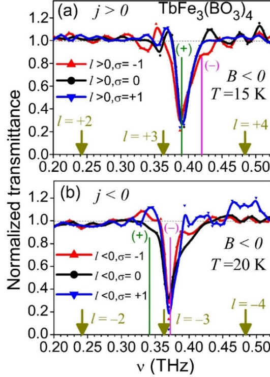
FIG. 3 (color online) Normalized transmittance spectra for the LG vortex beams for (a) j > 0 and (b) j < 0 in Tb-FB at B = -0.47 T. The resonance frequencies for \nu_{l=\pm 2} , \nu_{l=\pm 3} , and \nu_{l=\pm 4} are marked with bold dark yellow arrows. The temperatures were chosen to bring the AFM resonances \hbar\Omega_M^\pm(B, T) shown with vertical olive and magenta lines close to \nu_{l=\pm 3} in both, (a) and (b). Note that the corresponding AFM resonances coincide for j = +2 ( l = +3, \sigma = -1 ), j = +3 ( l = +3, \sigma = 0 ), and j = +4 ( l = +3, \sigma = +1 ) in (a) and for j = -2 ( l = -3, \sigma = +1 ), j = -3 ( l = -3, \sigma = 0 ), and j = -4 ( l = -3, \sigma = -1 ) in (b). The measurement geometry is the same as in FIG. 2(c) but with various input polarizations \vec{e}_y for black, \vec{e}_L for blue, and \vec{e}_R for red spectra.
