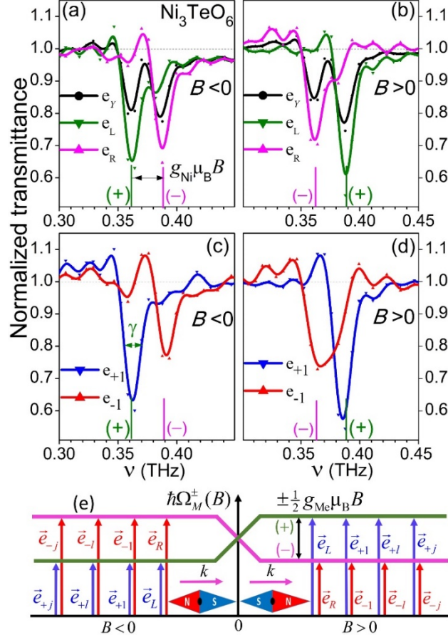
FIG. 1 (color online) Magnetic dichroism for circularly polarized light and vortex beams with l=\pm 1 in NTO. (a,b) Normalized transmittance for circularly polarized light, \vec{e}_L and \vec{e}_R , and for conventional linear polarization \vec{e}_y . (c,d) Normalized transmittance for broadband vortex beams with \vec{e}_{+1} (blue spectra) and \vec{e}_{-1} (red spectra). All experimental data in (a-d) are taken at B=\pm 0.47 T and T=10 K and are normalized to that measured at T=60 K in the same field: I(\nu, T)/I(\nu, T=60 \text{ K}) . (e) Schematics of the experimentally determined selection rules for the AFM resonances using both, circularly polarized light and vortex beams with l and j . The positive \vec{B} is parallel with \vec{k} .
