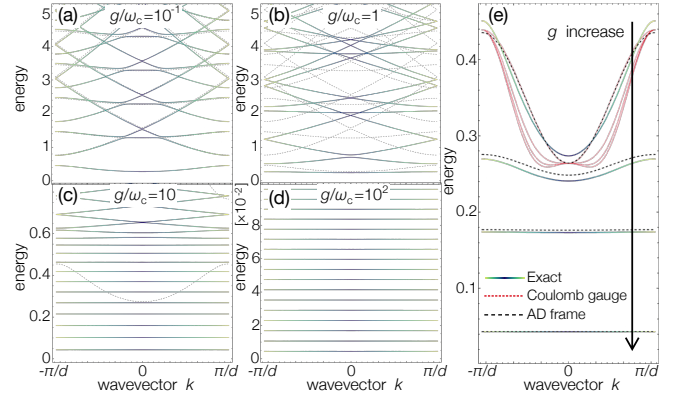
FIG. 2. (a-d) Exact electron-polariton bands obtained by diagonalizing Eq. (5). Gray dashed curves indicate dispersions at g = 0 . (e) Comparisons between the exact results and the tight-binding models at g = 0.1, 1, 2, 10 from top to bottom. Black dashed (red dotted) curves indicate the tight-binding results in the asymptotically decoupled frame (Coulomb gauge). We set v = 5 and d = 4 in (a-e).
