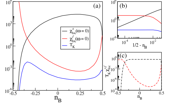
Figure 3. Evolution along the black NFL line in Fig. 1. (a) T = \omega = 0 susceptibilities \chi_{\text{loc}}^s (black), \chi_{\text{loc}}^f (red), and Kondo temperature T_K (blue). Flavor fluctuations are suppressed in the box Coulomb blockade regime, while spin fluctuations are suppressed as the dot local moment is lost for n_B \rightarrow -\frac{1}{2} . (b) Behavior near n_B = \frac{1}{2} showing \chi_{\text{loc}}^s(0) \sim (\frac{1}{2} - n_B)^2 (consistent with \chi_{\text{loc}}^s(\omega) \sim \omega ), while \chi_{\text{loc}}^f remains finite. (c) T_K \chi_{\text{loc}}^s (black dashed) and T_K \chi_{\text{loc}}^f (red dashed) showing crossover from spin-flavor to spin to flavor 2CK as n_B is varied from +\frac{1}{2} to -\frac{1}{2} .
