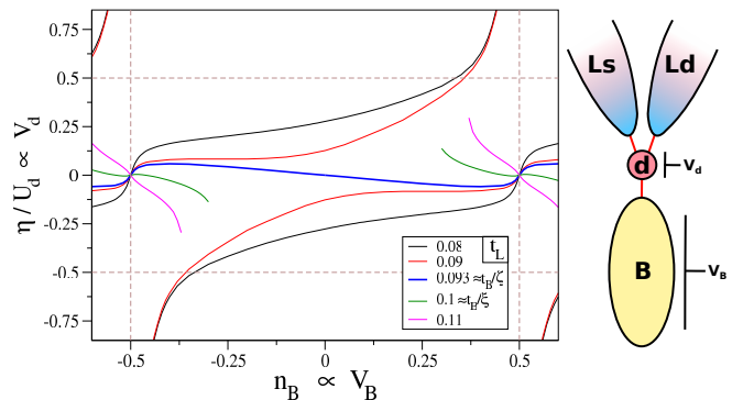
Figure 1. Right: Schematic of the device: a quantum dot coupled to a quantum box and source/drain leads. Left: NRG phase diagram spanned by dot and box gate voltages, V_d \propto \eta/U_d and V_B \propto n_B , showing the NFL line for various channel asymmetries t_L/t_B . SO(5) point located at n_B = \pm \frac{1}{2} and \eta = 0 . Plotted for constant U_d = 0.3 , E_C = 0.1 and t_B = 0.12 .
