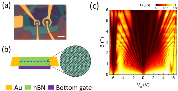
FIG. 1. Device structure and transport characterization. (a) Optical image of a Corbino geometry device. Scale bar: 10\mu m . (b) Schematic of the device structure: monolayer graphene sandwiched by hBN, with either a \text{SiO}_2/\text{Si} or graphite bottom gate. The moiré superlattice exists between monolayer graphene and either top or bottom hBN flake. (c) Characteristic Landau fan diagram of the monolayer graphene Corbino device C with moiré potential. Satellite conductance dips emerge at around V_g = \pm 6 V.
