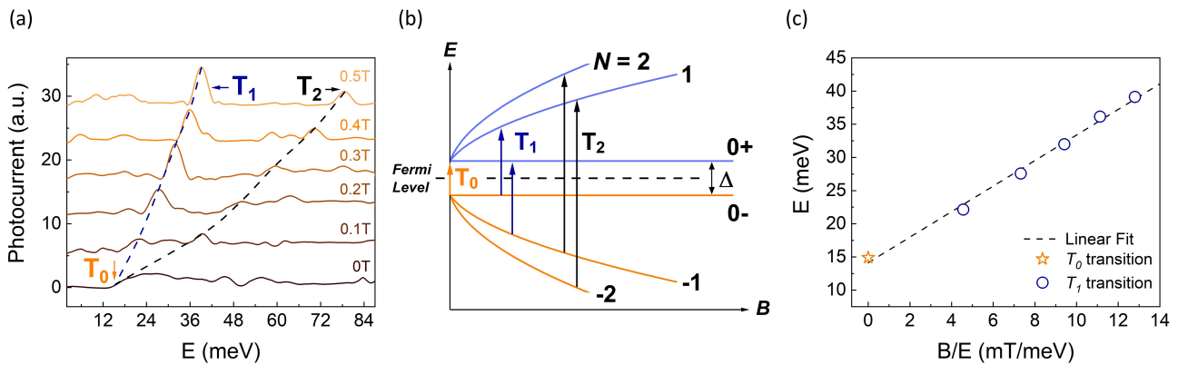
FIG. 2. Photocurrent spectra with the Fermi level located at the CNP. (a) Photocurrent spectra at magnetic field B = 0-0.5 T. At B = 0 T, the optical transition has a threshold energy of T_0 , which corresponds to the bandgap \Delta . When B increases, LLs are formed and inter-LL transitions labelled as T_1 and T_2 emerge from the continuous spectrum at 0 T. Spectra are shifted vertically for clarity. Dashed curves are guide lines of the T_1 and T_2 transitions. (b) Schematic illustrating the inter-LL transition T_1 and T_2 that are allowed by the optical selection rule \Delta|N| = \pm 1 . At the low magnetic field limit, they both converge to T_0 transition energy \Delta . (c) Extraction of \Delta from the fitting of T_0 (14.9 meV marked by star symbol in orange) and inter-LL transition T_1 by using E = 2e\hbar v_F^2 B/E + \Delta .
