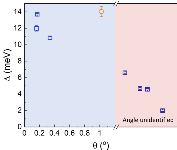
FIG. 4. Summary of the extracted gap sizes \Delta from devices with different moiré periods. The blue shaded area includes devices where the twist angle between graphene and hBN can be extracted from the satellite peak position in transport[39]. The pink shaded area includes devices with relatively large twist angles, which cannot be determined due to limited gate voltage range in experiment. Error bars show the standard deviations of multiple measurements at different magnetic fields. The orange circle data point is extracted via the first measurement scheme from device A, and other blue square data points are acquired via the second method.
