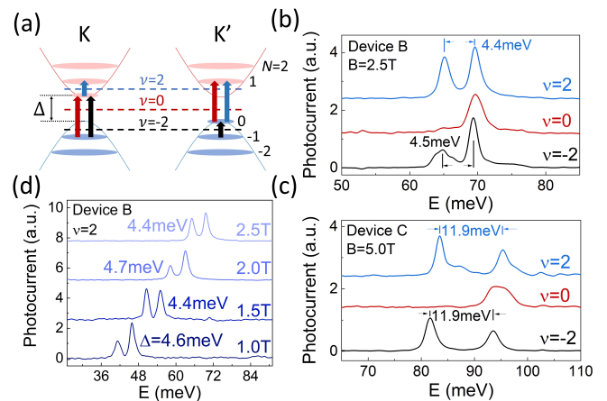
FIG. 3. Extraction of \Delta from inter-LL transitions at different filling factors. (a) Schematic showing allowed inter-LL transitions in the K and K' valleys of graphene when the Fermi level is adjusted to filling factor \nu = -2 (black dashed line and arrows), \nu = 0 (red) and \nu = 2 (blue). The zeroth LL is located at the bottom of the conduction band (top of the valence band) in the K (K') valley –lifting the valley degeneracy of inter-LL transitions. (b-c) Photocurrent spectra of device B at 2.5 T and device C at 5.0 T. In both cases, the two allowed inter-LL transitions remain degenerate at \nu = 0 , resulting in a single absorption peak. At both \nu = 2 & -2 , the two allowed transitions are split by the gap energy \Delta . Transitions at \nu = 2, 0, -2 correspond to blue, red and black arrows in (a) respectively. (d) Photocurrent spectra at \nu = 2 for device B as a function of magnetic field from 1.0 T to 2.5 T. The splitting between two inter-LL transitions in all spectra are close to 4.5 meV as labelled.
