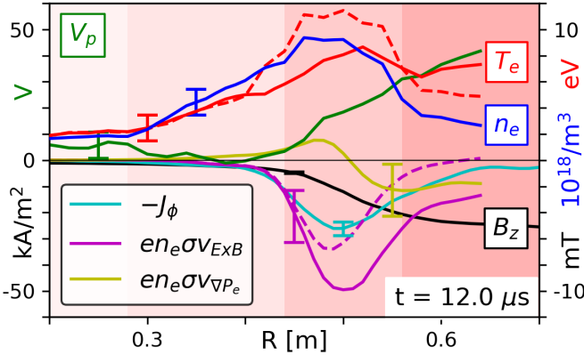
FIG. 3. R-profile at z=0.05 m, t=12 \mu\text{s} showing n_e , T_e , and V_p from Langmuir measurements, and J_\phi and B_z from magnetic measurements. Error bars show total error, not shot-to-shot uncertainty, which is small. The four colored areas left to right show the upstream, foot, layer, and downstream regions. The dashed red line is an adiabatic heating model, T_e = T_{e0}(n_e/n_0)^{\gamma-1} , for \gamma = 2 . The factor \sigma \equiv \omega_{ce}^2/(\nu_e^2 + \omega_{ce}^2) is an experimental parameter that accounts for collisional slowing [26]. The dashed magenta line estimates the sum current of the electron and ion \mathbf{E} \times \mathbf{B} \hat{\phi} drifts, which is zero in MHD. Within error, the measured toroidal current is the sum of the \mathbf{E} \times \mathbf{B} \hat{\phi} and electron diamagnetic drifts.
