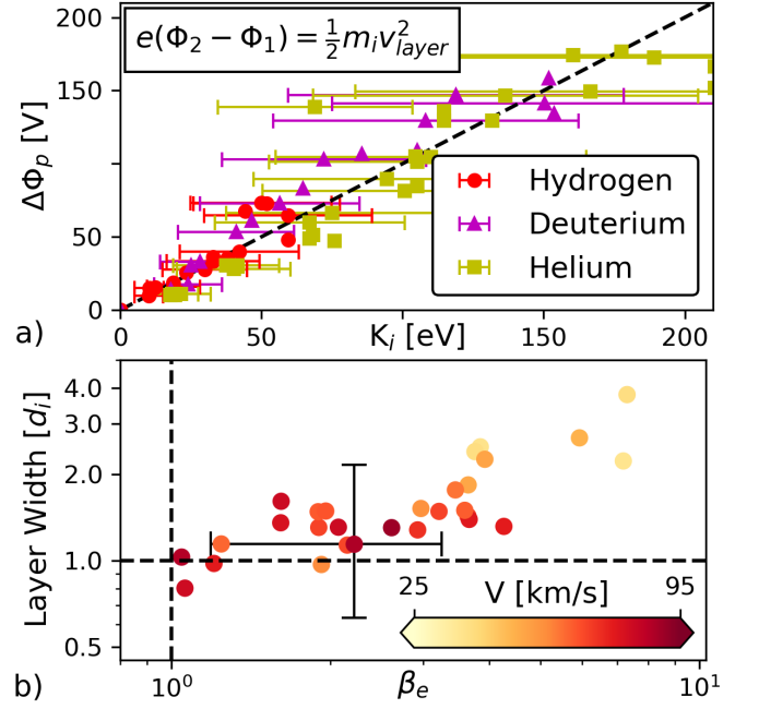
FIG. 4. a) Plasma potential jump \Delta\Phi_p vs convected ion kinetic energy K_i = 1/2 m_i v_l^2 showing a 1:1 relationship. \Delta\Phi_p was measured a distance of d_i/2 on either side of the layer peak with both emissive and Langmuir probes. b) Current layer thickness against \beta_e in the current layer for a variety of drive strengths in \text{H}_2 . As the magnetic piston becomes larger, the relative \beta_e decreases, leading to weaker \nabla B drifts and a thinner current layer.
