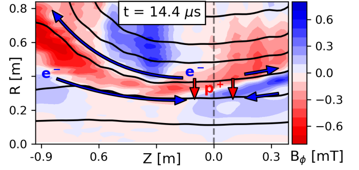
FIG. 5. Profile of toroidal magnetic field with arrows indicating direction of electron and ion flows. The red lobe at (z, r) = (-0.8, 0.5) \text{ m} implies current in the clockwise direction, consistent with an electron flow needed to maintain \nabla \cdot \mathbf{J} = 0 . The peak of the toroidal current layer is near the base of the red arrows. The axial density gradient from plasma injection at the +\hat{z} north pole skews the quadrupole slightly to the south.
