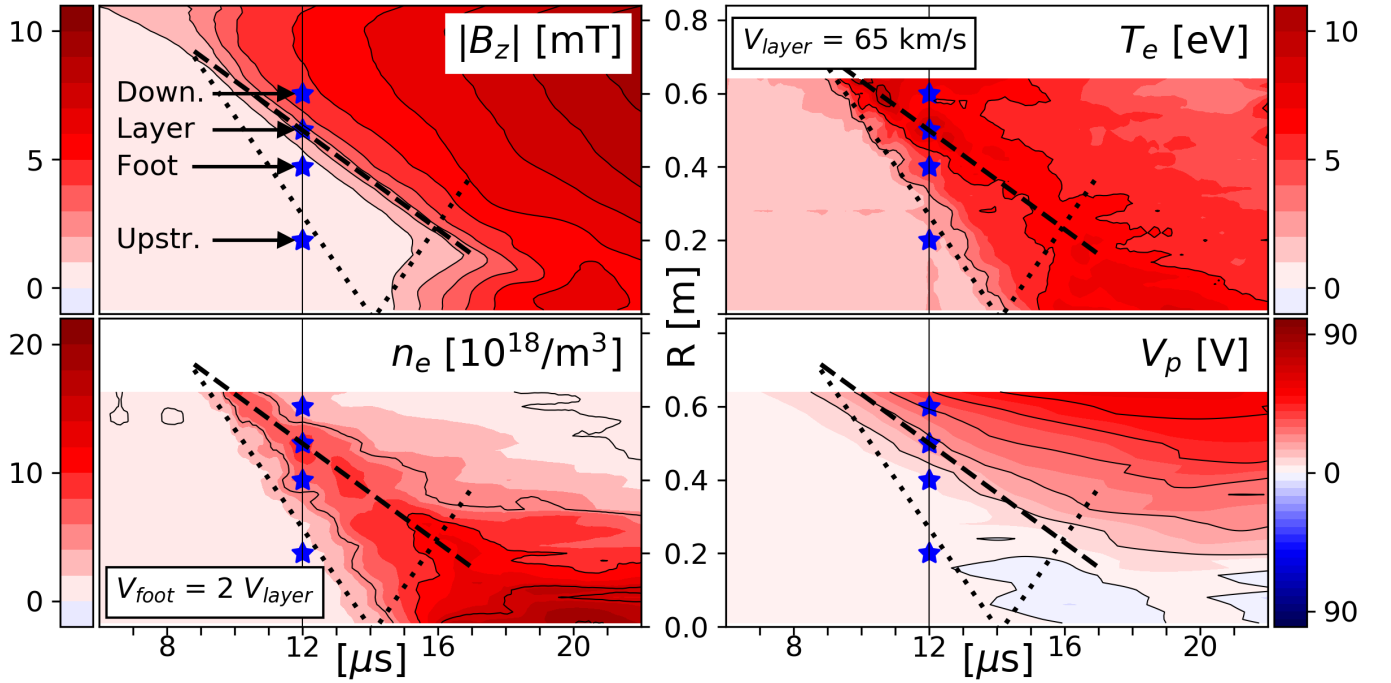
FIG. 2. Magnetic and Langmuir probe measurements of radially imploding \theta -pinch. This slice is taken at z=0.05 m, parallel to the “Radial Probe” in Fig. 1. The black dashed line is a linear fit to the peak of the toroidal current layer, with the dotted lines plotted for convenience at twice the speed. Note that the dotted lines border the earliest rise in density and temperature, and that the “reflection” through the axis aligns with an increase in B_z . Values from the starred locations are listed in Table I, and data along the line at t = 12 \mu\text{s} are shown in Fig. 3. The radial electric field E_r = -\nabla_r V_p is strongest along the current layer, as seen in Fig. 3. The drop in potential after 12 \mu\text{s} is a result of boundary conditions and electron heating in the foot, but does not affect E_r in the layer.
