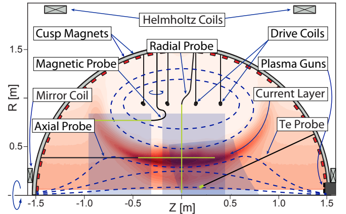
FIG. 1. Experimental cross section. Blue shaded regions show the coverage of the Langmuir probe (wedge) and magnetic probes (rectangles). The red contour map qualitatively depicts the density during \theta -pinch compression, with blue dashes showing selected magnetic field lines. The four drive coils can be seen at R = 92 cm, Z = \pm 15, \pm 40 cm. Washer guns on axis supply the background plasma, which in the mirror configuration exhibits a relatively flat initial radial density profile.
