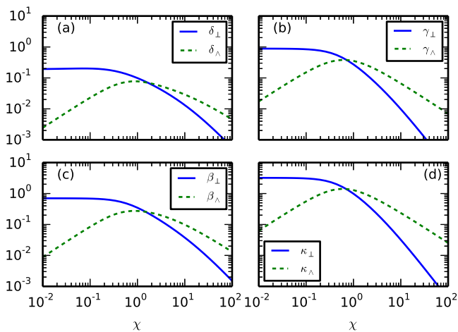
FIG. 2: The symmetric form of the transport coefficients for \bar{Z} = 1 . (a) The Hall coefficients \delta_\perp and \delta_\Lambda . (b) The Nernst coefficients \gamma_\perp and \gamma_\Lambda . (c) The thermoelectric coefficients \beta_\perp and \beta_\Lambda . (d) The Spitzer coefficients \kappa_\perp and \kappa_\Lambda .
