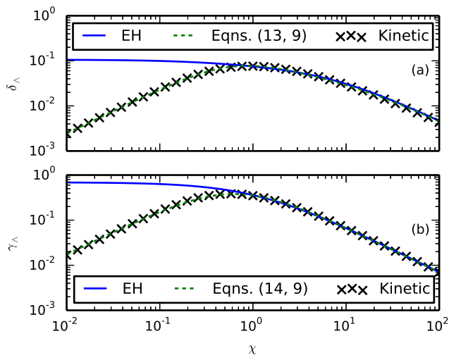
FIG. 1: Plots of the kinetic (a) \delta_\Lambda cross-Hall and (b) \gamma_\Lambda cross-Nernst transport coefficients for \bar{Z} = 1 , fitted using eqns. (13-14) in eqn. (9). The results of Epperlein and Haines (EH) [15] are only accurate for \chi > 1 .
