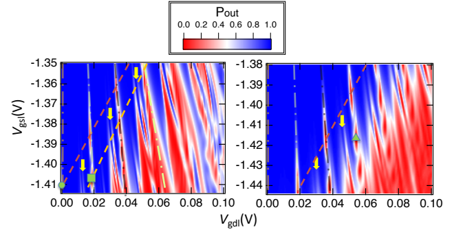
FIG. 3. Numerically calculated probability P_{out} of electron staying in the lower wire through the TCR. Left: Typical result when electrons are fully trapped by the SAW potential during the time evolution. V_c = -1 V, V_{fl1} = V_{fl2} = -1.1 V, V_{bl1} = V_{bl2} = -1.2 V. Right: typical result when a part of electrons drop off the SAW potential at the middle of the TCR. V_c = -1 V, V_{fl1} = V_{fl2} = -1.1 V, V_{bl1} = V_{bl2} = -1 V.
