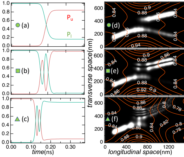
FIG. 4. Calculated temporal and spatial distribution of an electron in the TCW for each marked point in Fig.3. (a)–(c): Probability of finding an electron in the lower channel, P_l in green and upper channel, P_u in red, respectively at each time instance. (d)–(f): Cumulative SPDs of those obtained at the time intervals of 15.4 ps with contour plots of the potential profile.
